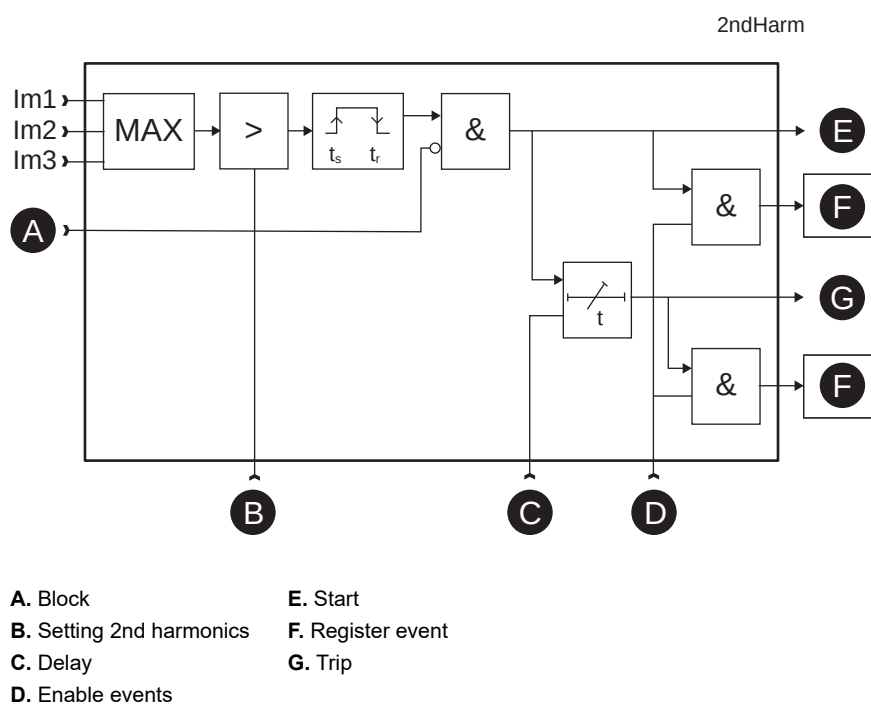
Figure 129 - Block diagram of the magnetizing inrush detection stage
