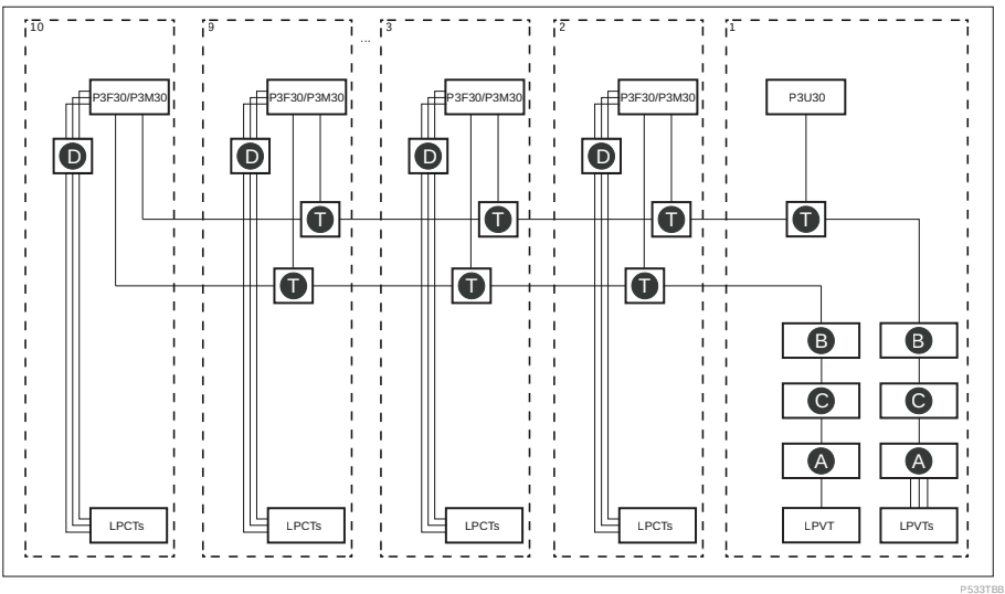
Figure 273 - LPVT sharing application including the 4 th voltage (sync-check) and with test sockets/plugs
