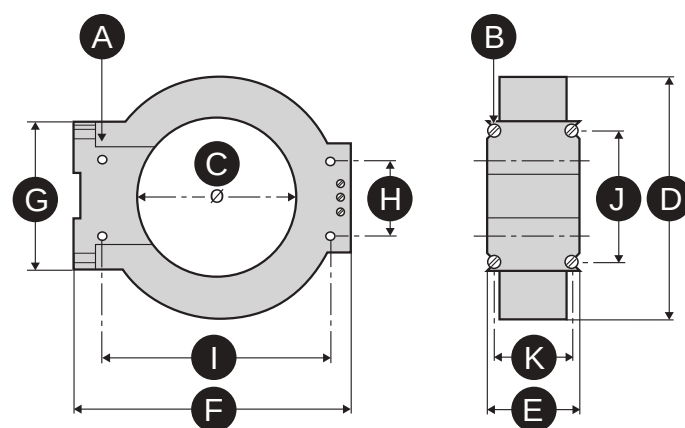
Figure 293 - Dimensions
