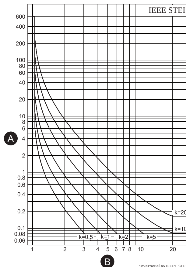
Figure 66 - ANSI/IEEE short time extremely inverse delay
