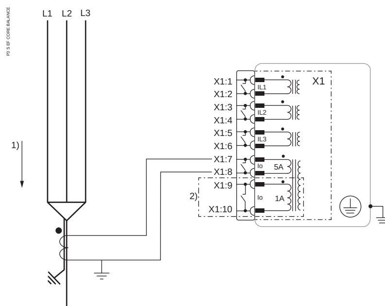
Figure 228 - Earth fault overcurrent by core balance CT
