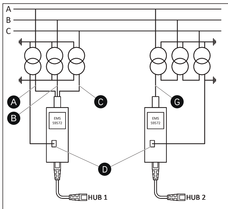
Figure 241 - 3LN+U 0 connection
