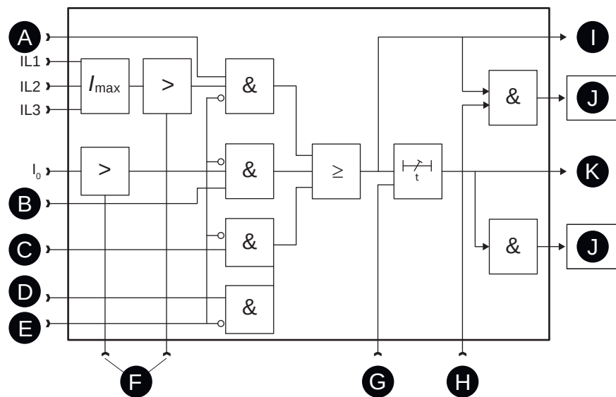
Figure 89 - Breaker failure 2 operation
