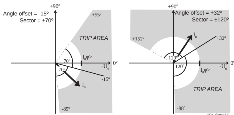
Figure 123 - Operation characteristics examples of the directional earth fault stages in the sector mode
