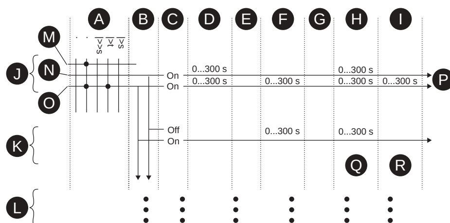
Figure 132 - Auto-recloser matrix
