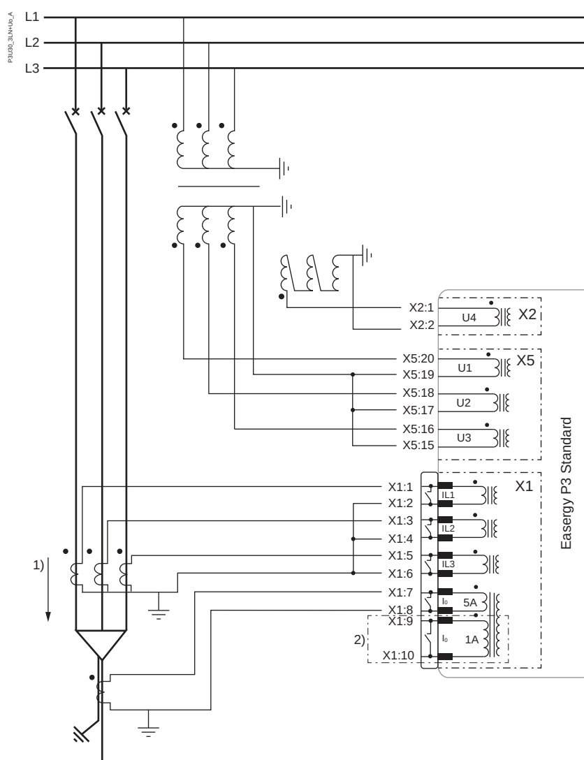
Figure 233 - 3LN voltages + U 0 + 3LN currents + core balance EF
