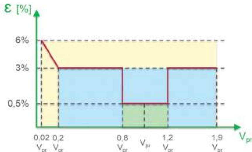
Figure 259 - Magnitude accuracy
