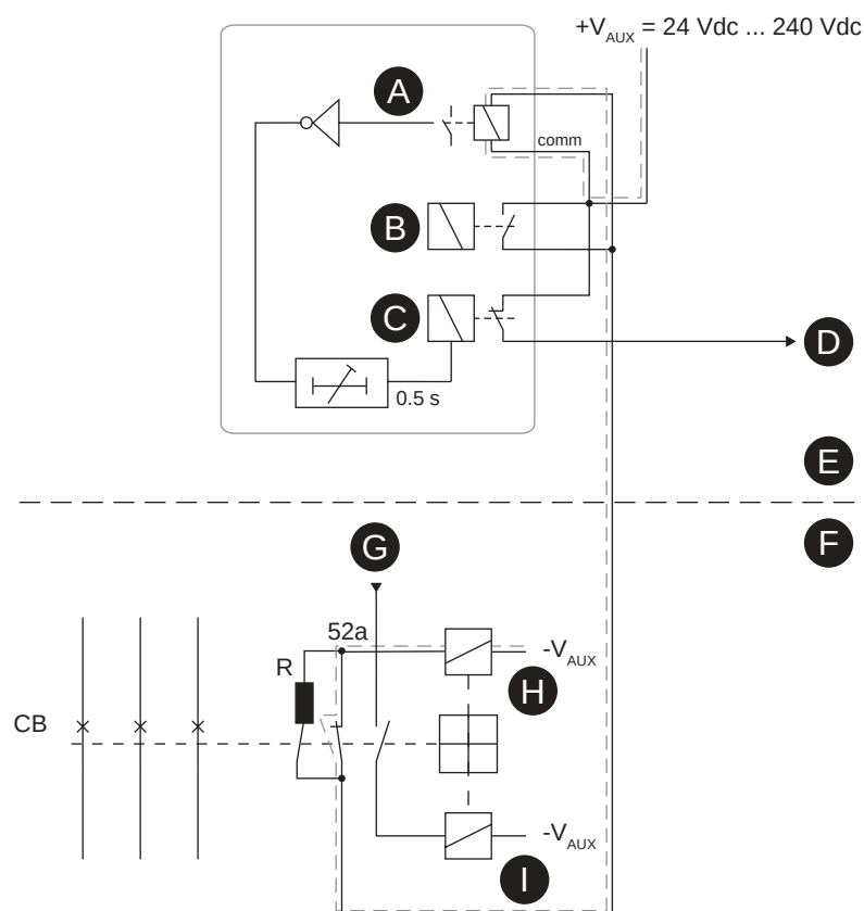
Figure 166 - Alternative connection without using circuit breaker 52b auxiliary contacts
