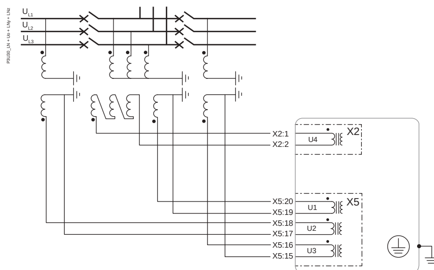
Figure 289 - LN+U 0 +LNy+LNz
