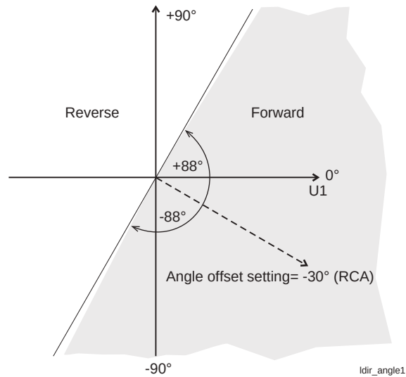
Figure 116 - Example of the directional phase overcurrent protection area for line-to-line fault
