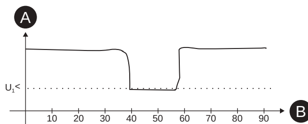
Figure 146 - A short voltage interruption which is probably not recognized
