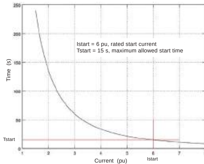
Figure 79 - Example of a dependent operate time delay of the motor start-up supervision stage
