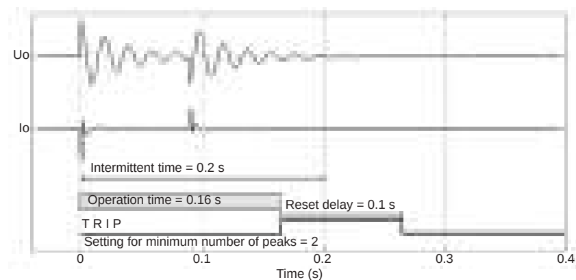
Figure 125 - Set peak amount is satisfied and operate time comes full inside intermittent time setting. Stage issues a trip.
