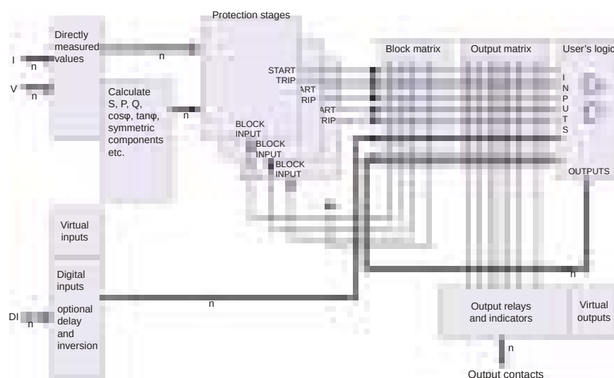
Figure 27 - Blocking matrix and output matrix
