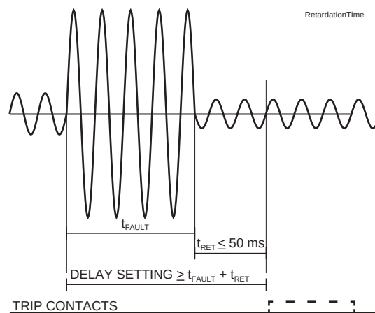
Figure 52 - Overshoot time
