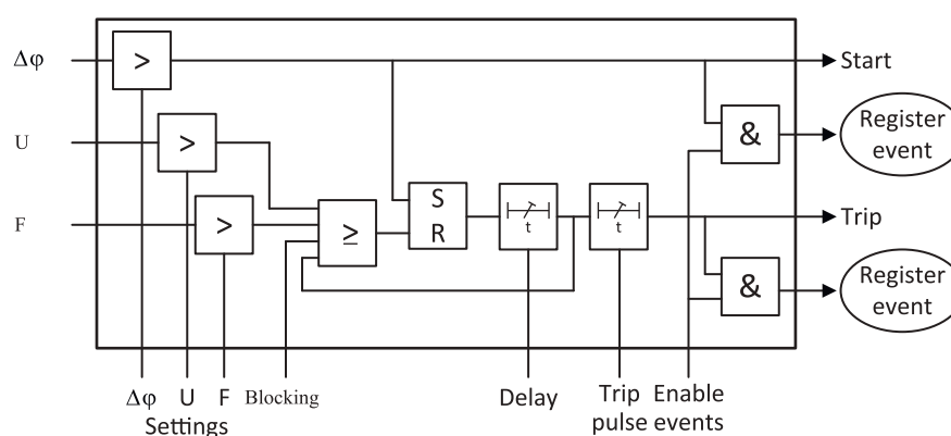
Figure 130 - Logic of the vector shift protection
