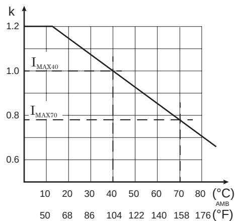
Figure 85 - Ambient temperature correction of the overload stage T>
