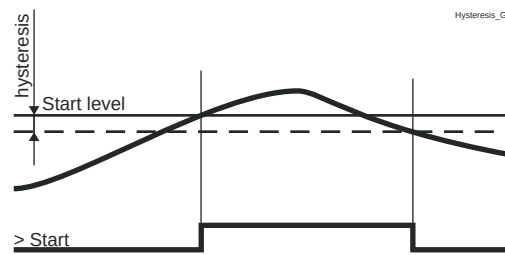
Figure 54 - Example behavior of an over-protection with hysteresis
