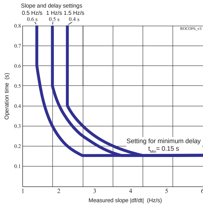
Figure 136 - Three examples of possible dependent df/dt operate time characteristics. The slope and operation delay settings define the knee points on the left. A common setting for t_{Min} has been used in these three examples. This minimum delay parameter defines the knee point positions on the right.
