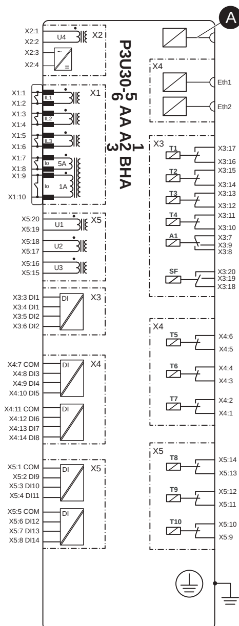
Figure 223 - P3U30 5AA A1BHA block diagram
