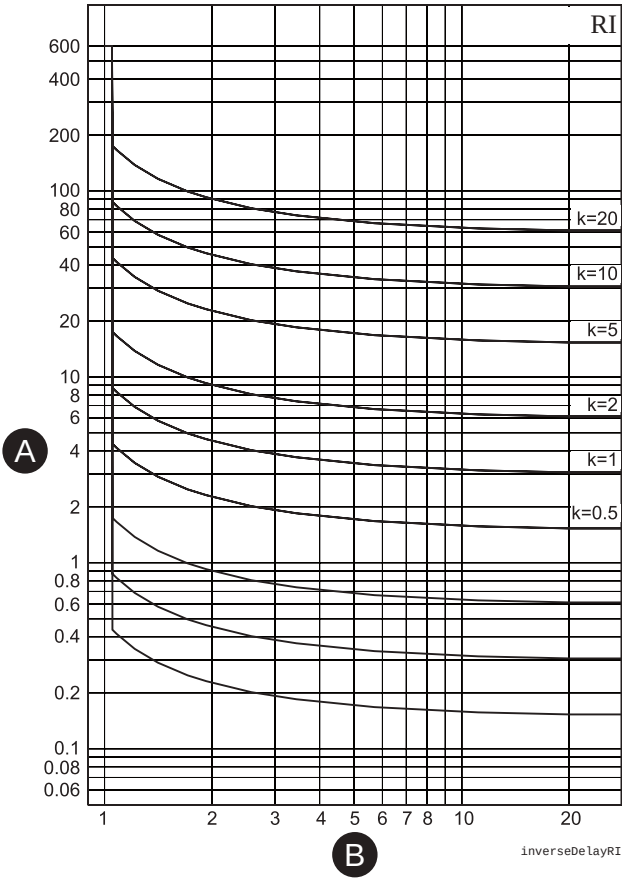
Figure 71 - RI dependent delay
