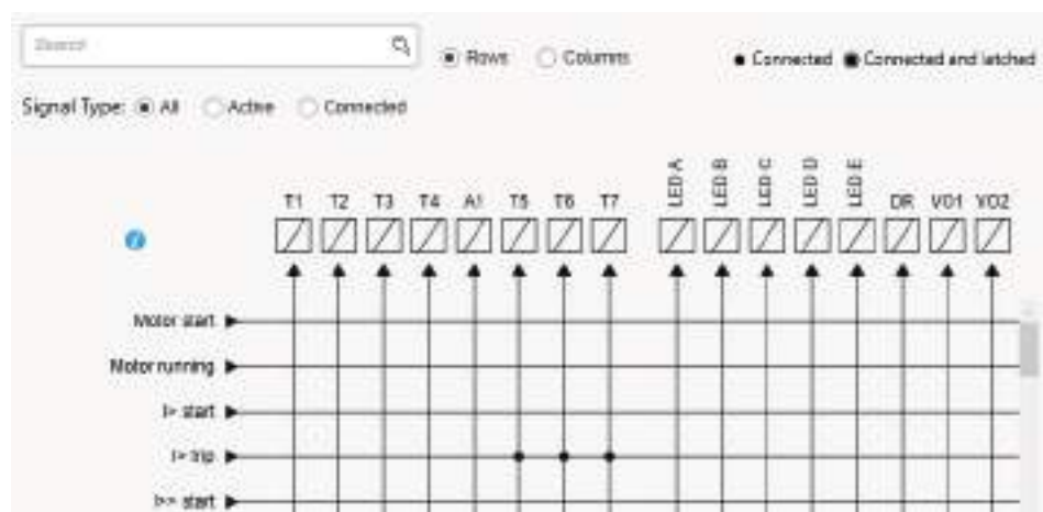
Figure 12 - Output matrix view
