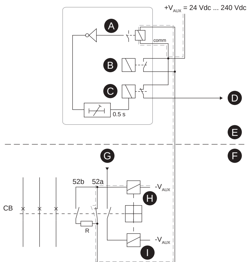
Figure 165 - Trip circuit supervision using a single digital input and an external resistor R
