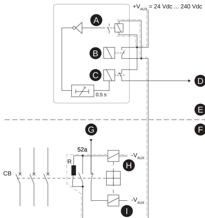
Figure 168 - Alternative connection without using circuit breaker 52b auxiliary contacts. Trip circuit supervision using a single digital input, when the circuit breaker is in open position
