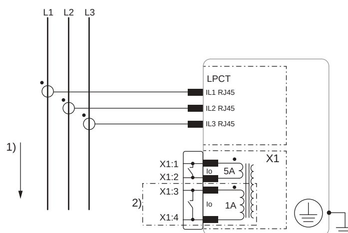
Figure 234 - Three-phase current measurement with LPCTs
