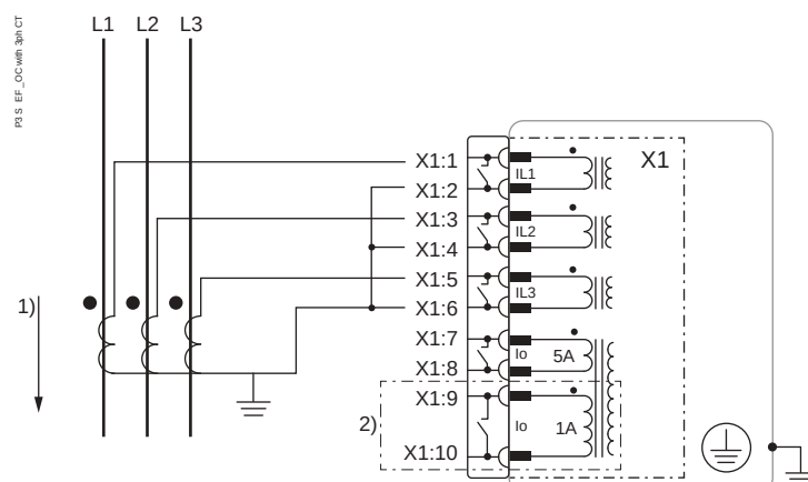
Figure 226 - Three-phase current measurement
