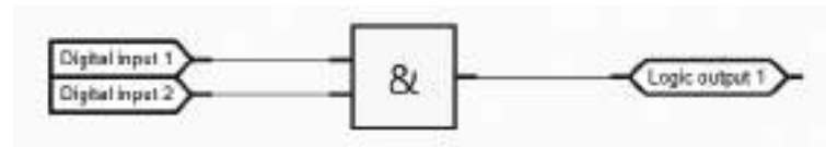
Figure 174 - An example of logic configuration for trip circuit supervision with two digital inputs DI1 and DI2.
