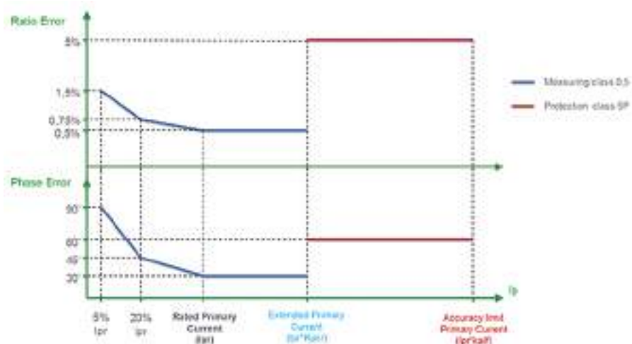
Figure 253 - Magnitude and phase errors across the measurement range
