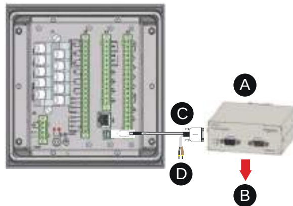
Figure 213 - VPA-3CG module
