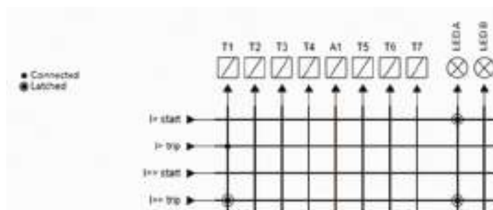
Figure 138 - The lockout programmed for LED A and I>> trip signals
