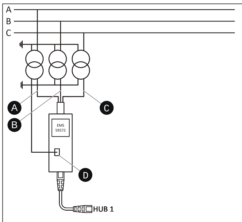
Figure 239 - 3LN connection
