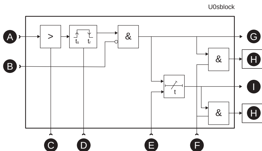
Figure 112 - Block diagram of the neutral voltage displacement stages U_0> , U_0>> , U_0>>>
