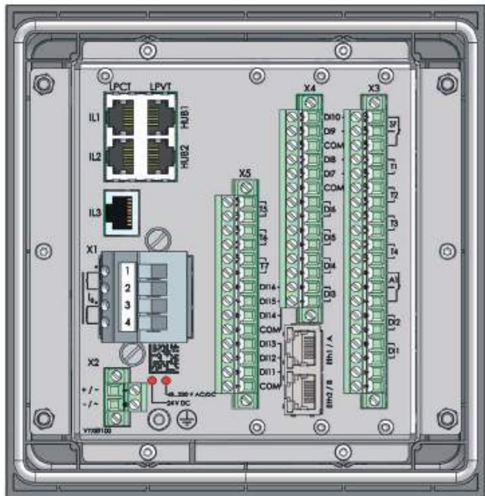
Figure 237 - P3U rear panel – LPIT
