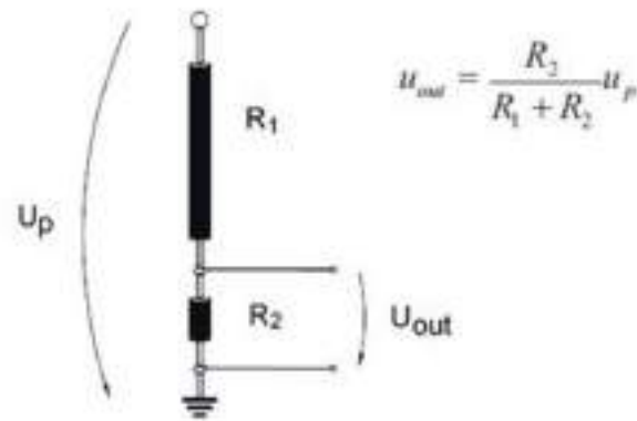
Figure 266 - Resistive divider
