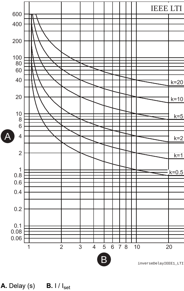
Figure 61 - ANSI/IEEE long time inverse delay
