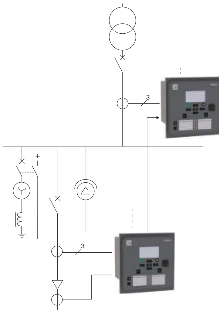
Figure 191 - PowerLogic P3U20 and P3U30 used in substation feeder protection in compensated network
