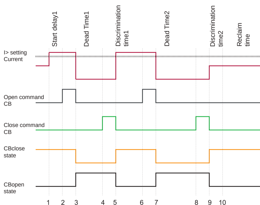
Figure 133 - Example sequence of two shots. After shot 2, the fault is cleared.
