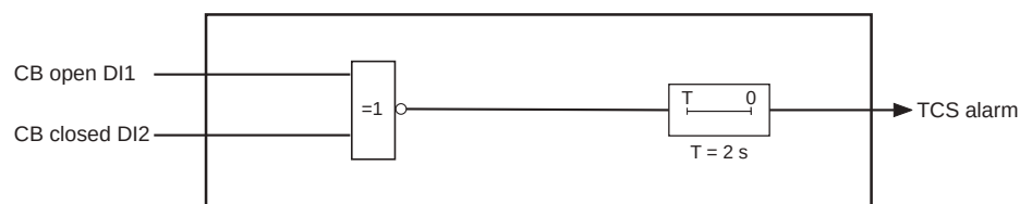
Figure 177 - Block diagram of trip circuit supervision (ANSI 74)
