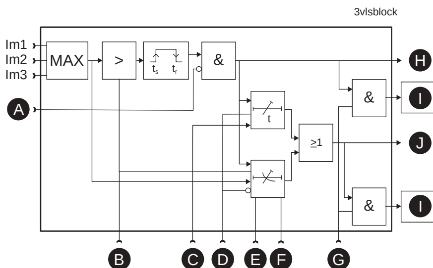
Figure 94 - Block diagram of the three-phase overcurrent stage I >
