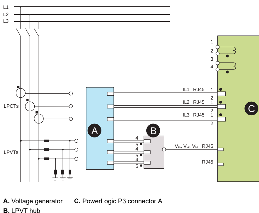
Figure 274 - Connection diagram for testing the LPIT
