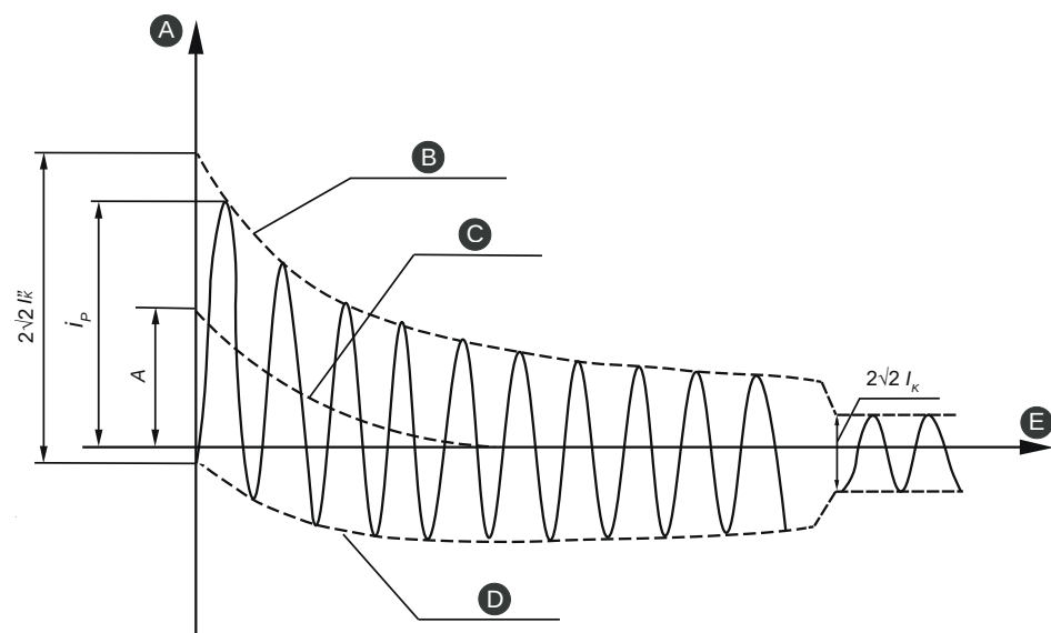
Figure 254 - Fault characteristic
