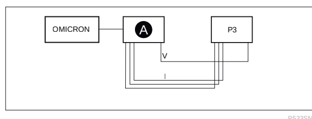
Figure 278 - LPCT/LPVT direct testing without test sockets/plugs
