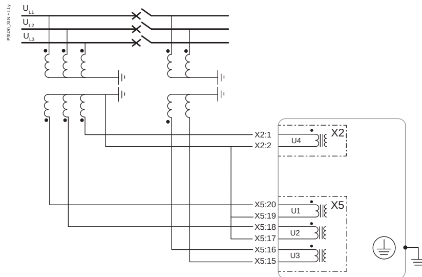
Figure 283 - 3LN+LLy
