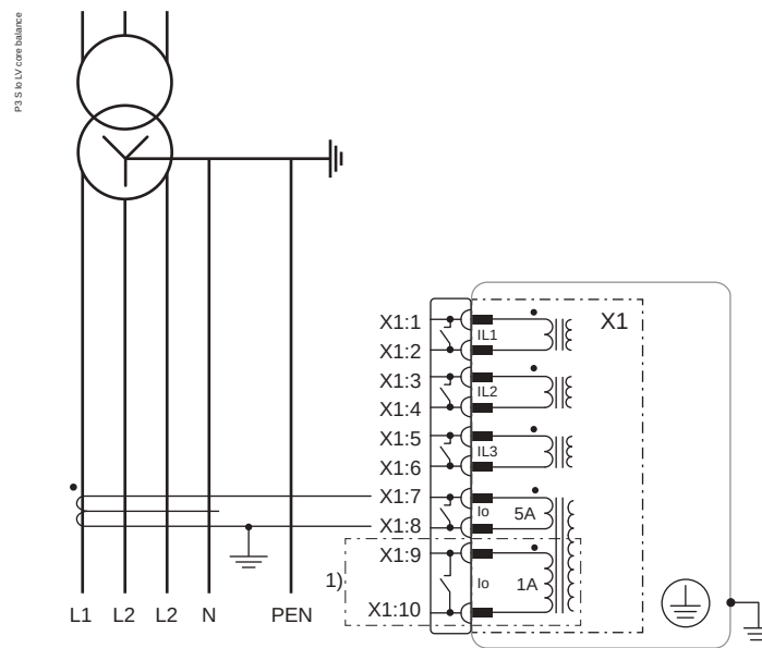
Figure 231 - Earth fault overcurrent measurement by using core balance CT
