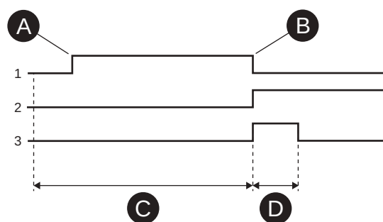
Figure 76 - Synchrocheck function principle
