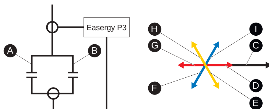
Figure 100 - How a failure in different branches of the bank affects the I_0 measurement
