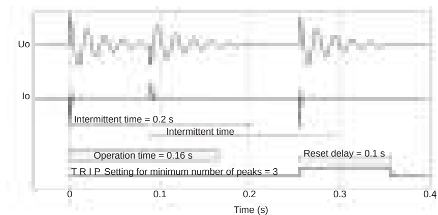
Figure 126 - Peak amount is not satisfied when operation delay comes full but last required peak comes during intermittent time. Stage issues instant trip when peak amount comes satisfied.
