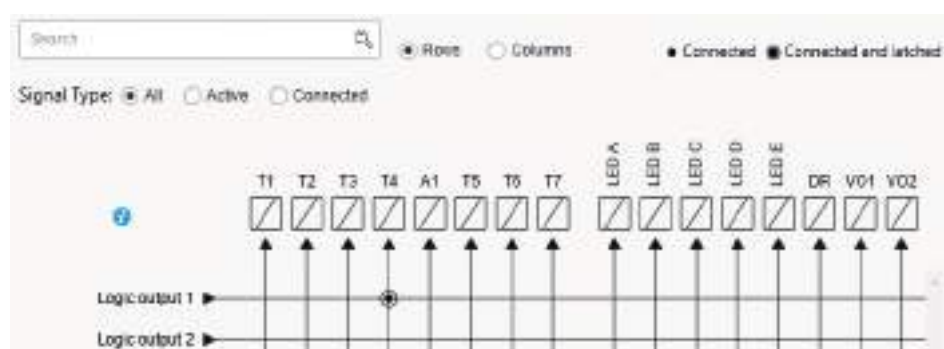
Figure 13 - Trip contacts assigned directly to outputs of logical operators
