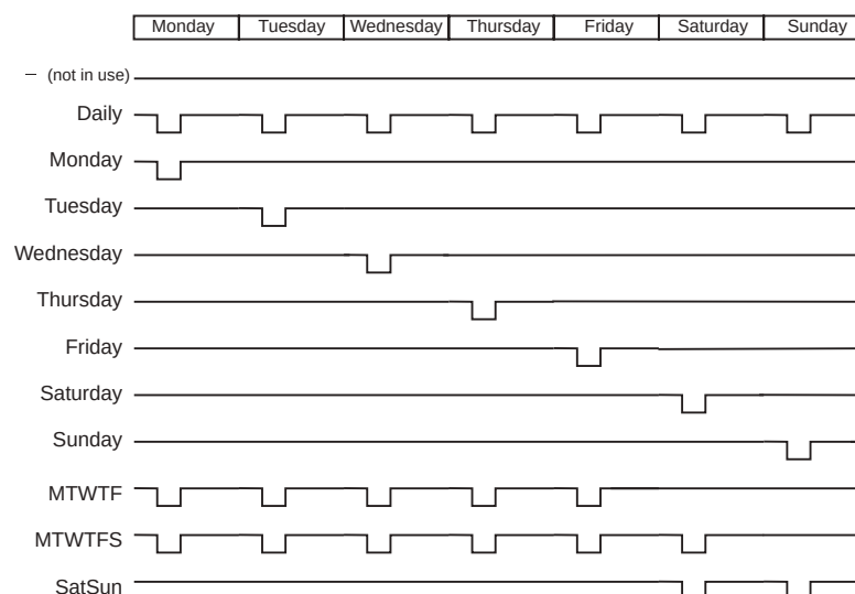
Figure 160 - Timer output sequence in different modes
