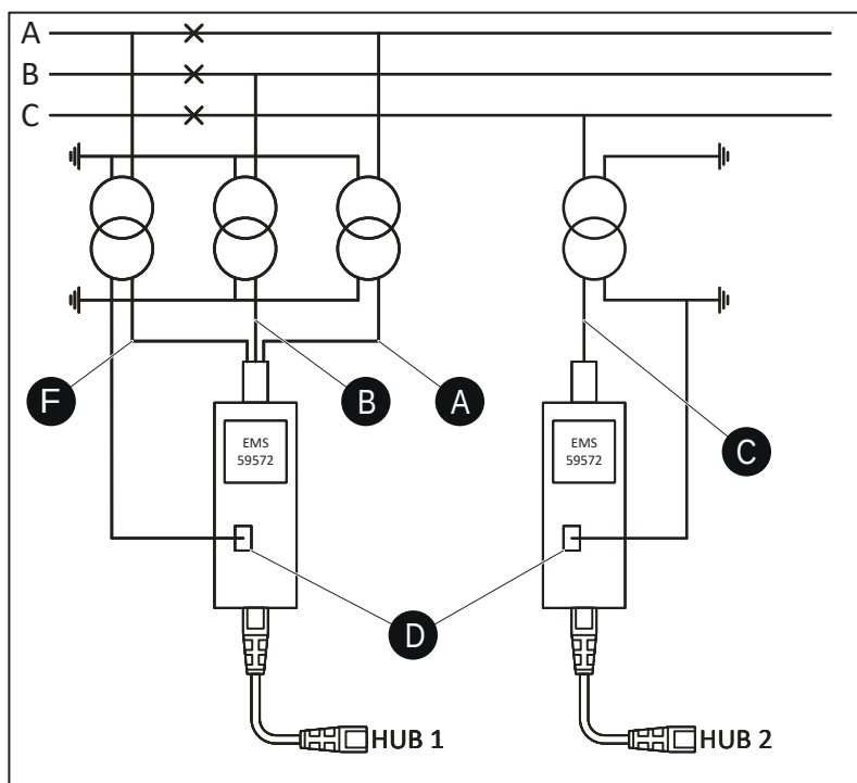
Figure 240 - 3LN/LNy connection
