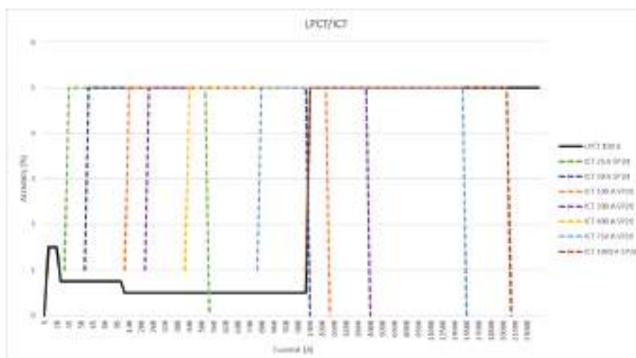
Figure 252 - LPCT protection accuracies for primary currents
