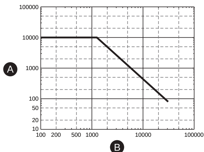
Figure 149 - Example permissible cycle diagram
