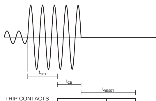
Figure 53 - Reset time
