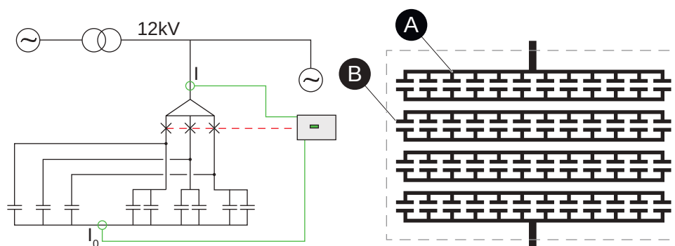
Figure 101 - 131.43 \mu\text{F} Y-Y connected capacitor bank with internal fuses
