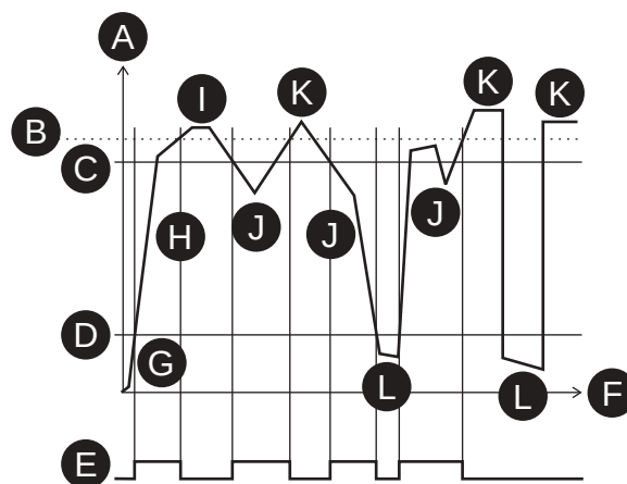
Figure 77 - Example of low-voltage self blocking
