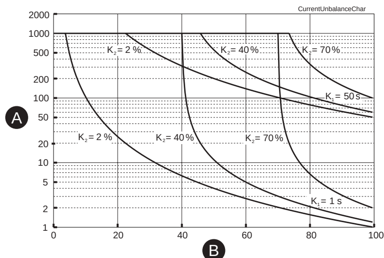
Figure 78 - Dependent operation delay of negative sequence overcurrent I_2 > (ANSI 46). The longest delay is limited to 1000 seconds (=16min 40s).
