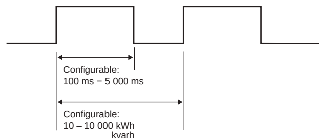
Figure 156 - Principle of energy pulses
