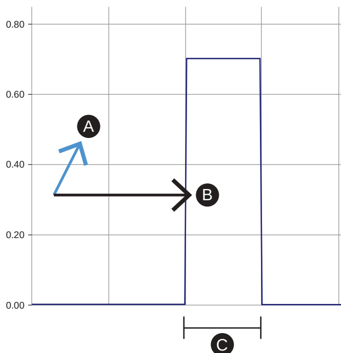
Figure 104 - Testing the operation of the unbalance protection
