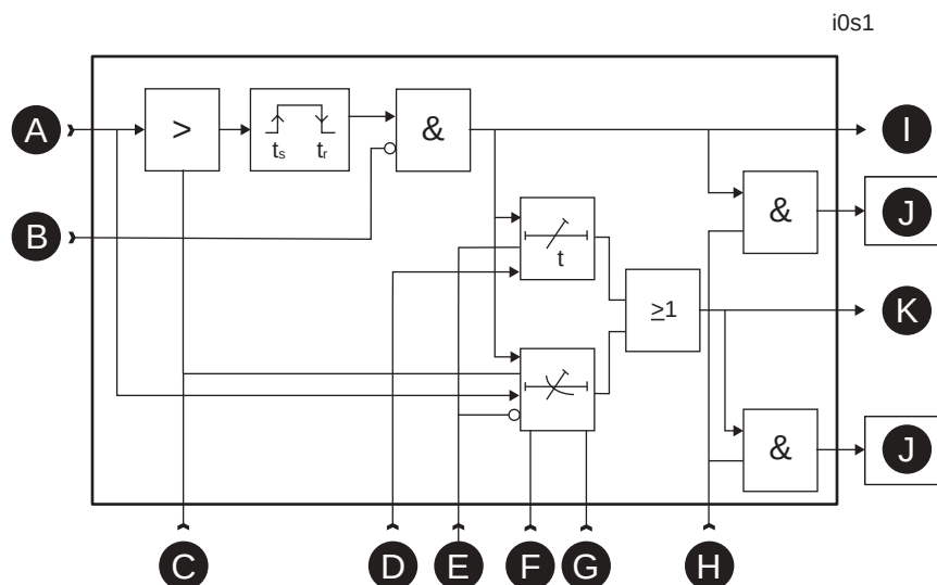
Figure 96 - Block diagram of the earth fault stage overcurrent I_{0>}
