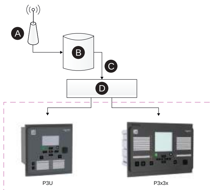
Figure 145 - PowerLogic P3 relays with IRIG-B synchronization capability
