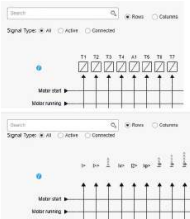
Figure 82 - Motor status in output and block matrix
