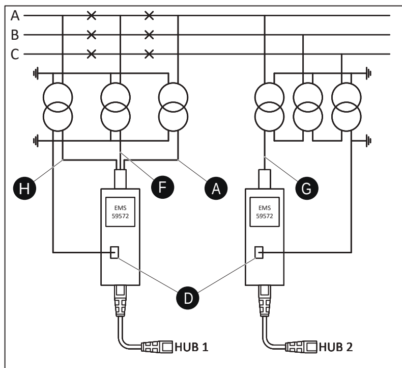
Figure 242 - LN+U 0 /LNy/LNz connection
