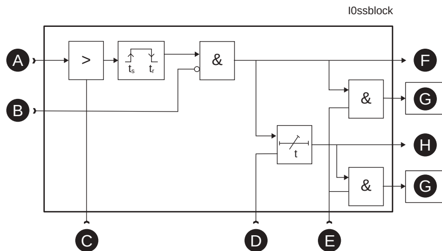
Figure 97 - Block diagram of the earth fault stages overcurrent I_0>> , I_0>>> , I_0>>>> , I_0>>>>>
