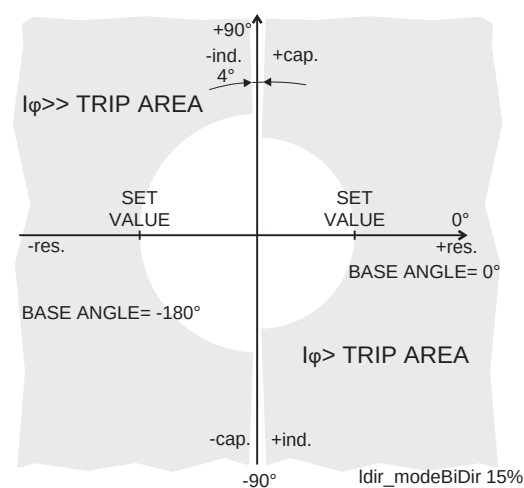
Figure 119 - Bidirectional application with two stages I_{\varphi>} and I_{\varphi>>}
