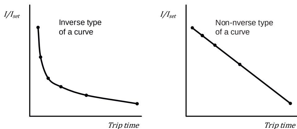
Figure 73 - Inverse and non-inverse curve
