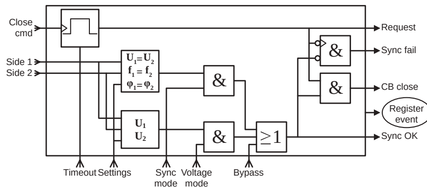
Figure 74 - Synchrocheck function
