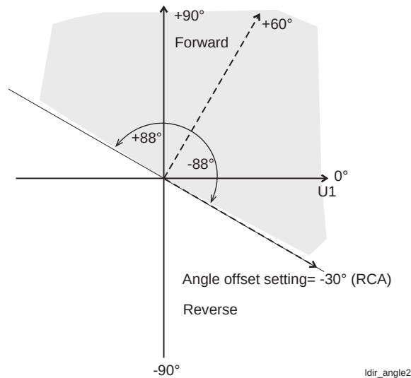
Figure 117 - Example of the directional phase overcurrent protection area for line-to-earth fault , RCA internally rotated +90^\circ CCW during earth fault
