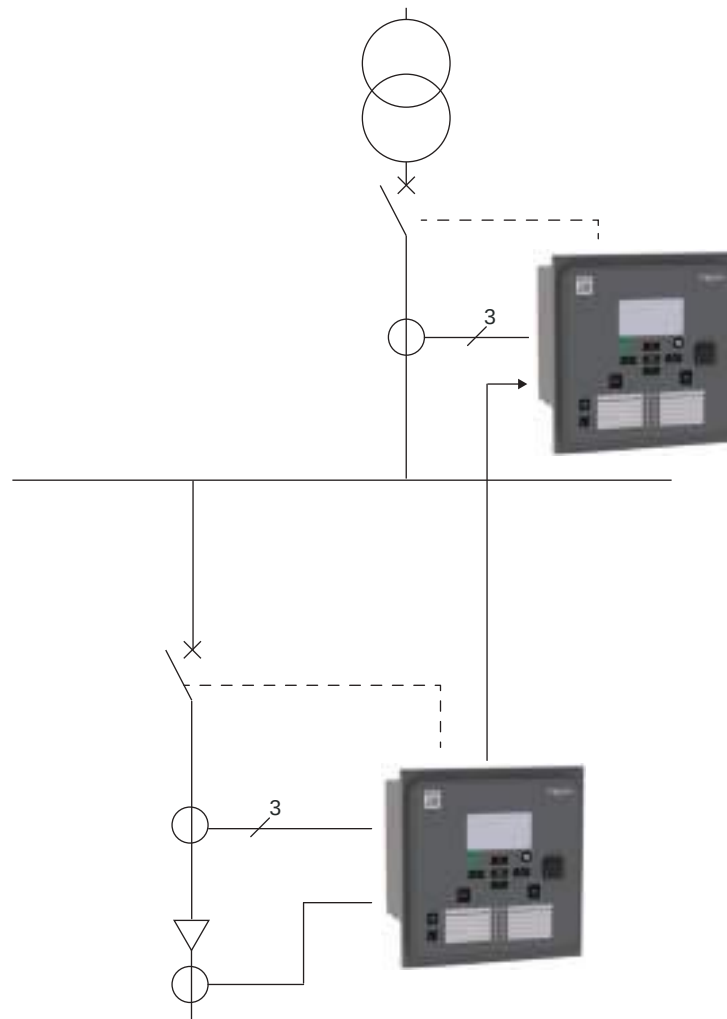
Figure 190 - PowerLogic P3U20 and P3U30 used in substation feeder protection
