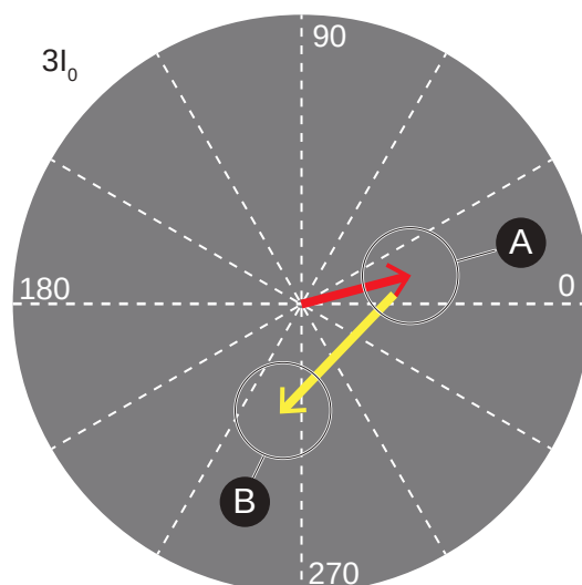
Figure 99 - Natural unbalance compensation and a single capacitor fault
