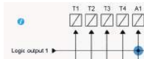
Figure 175 - An example of output matrix configuration for trip circuit supervision with two digital inputs
