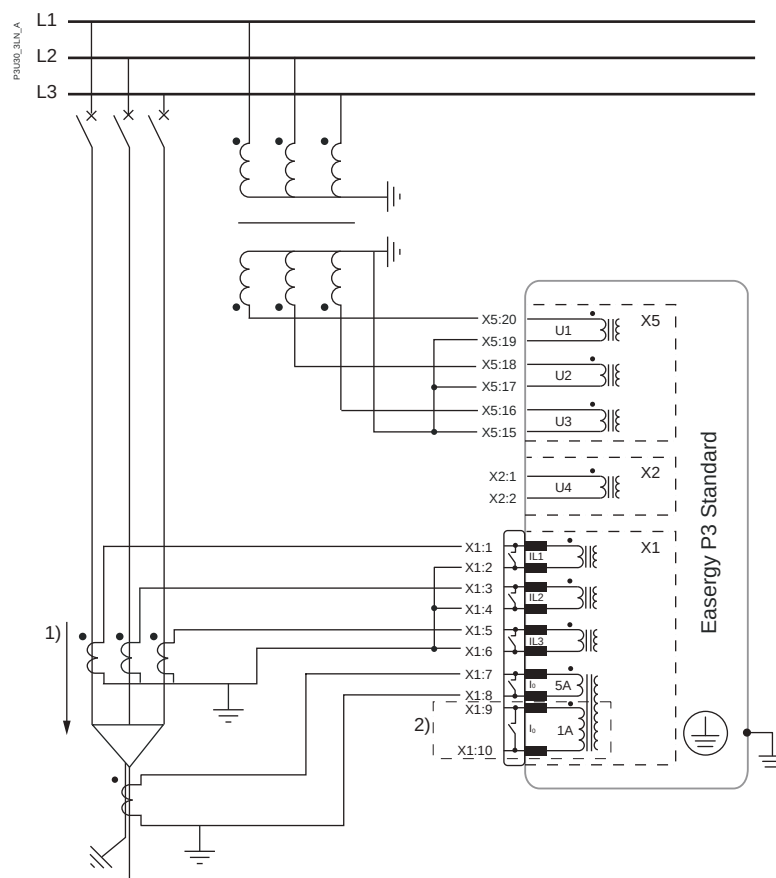
Figure 232 - 3LN voltages + 3LN currents + core balance EF
