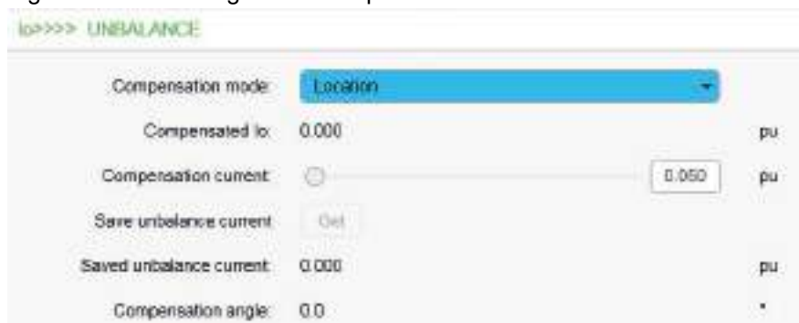
Figure 102 - Enabling unbalance protection
