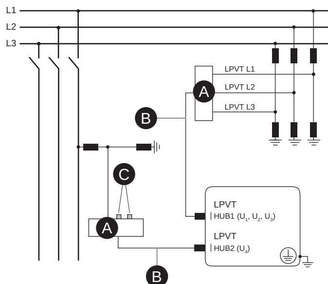
Figure 236 - Three line-to-neutral LPVTs + one line-to-neutral LPVT
