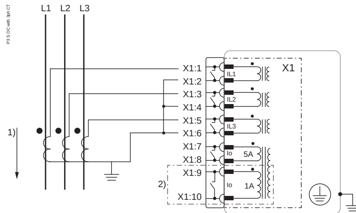
Figure 227 - Earth fault overcurrent calculation from phase currents
