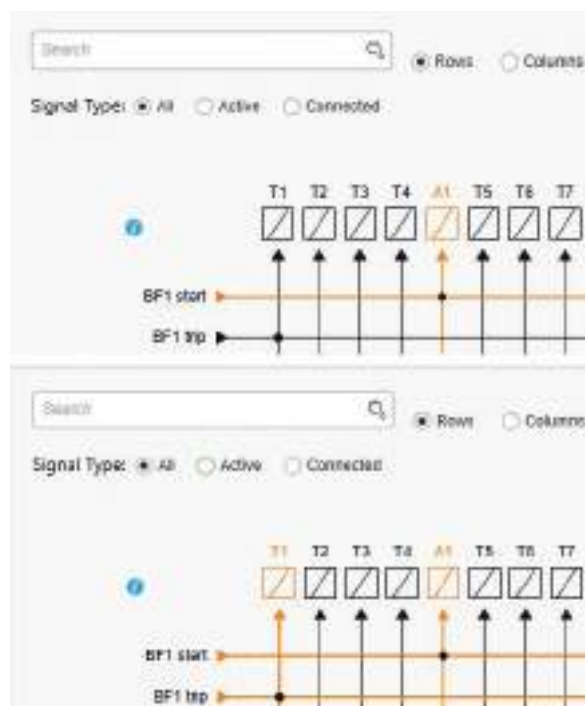
Figure 87 - Trip and CBFP start signals in the Output matrix view
