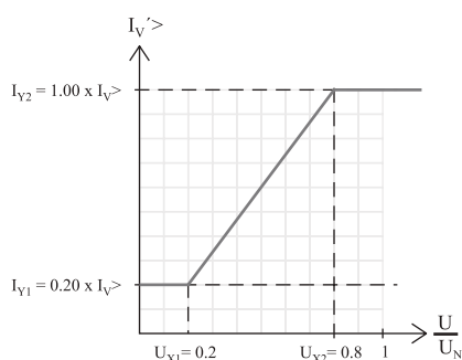
Figure 107 - Characteristics of the voltage-restrained overcurrent function I_V>
