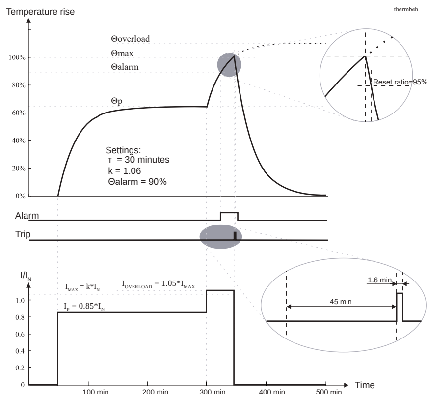
Figure 86 - Example of the thermal model behavior
