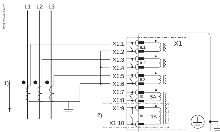
Figure 225 - Three-phase current measurement
