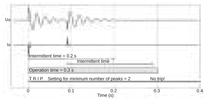
Figure 127 - Peak amount is satisfied but intermittent time comes full before operate time comes full. Stage is released.
