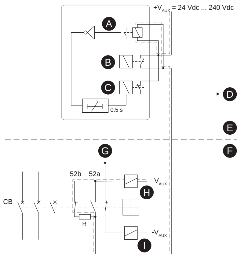
Figure 167 - Trip circuit supervision using a single digital input when the circuit breaker is in open position
