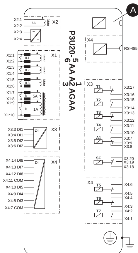
Figure 218 - P3U20 5AA A1AGAA block diagram
