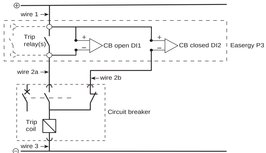
Figure 176 - Trip circuit supervision scheme
