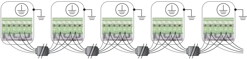
Figure 208 - RS-485 multidrop connections
