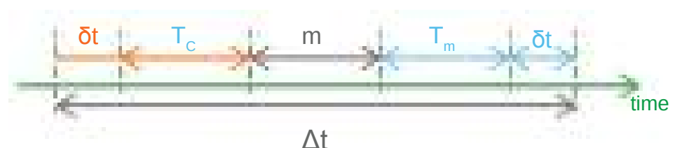
Figure 56 - Time grading
