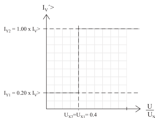
Figure 108 - Voltage-controlled overcurrent characteristics
