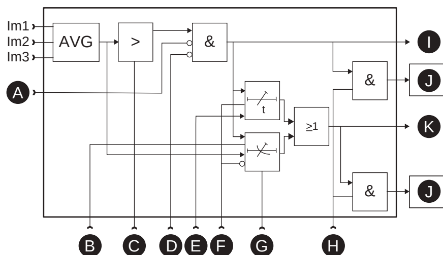
Figure 106 - Block diagram of the locked rotor protection stage I_{lr}
