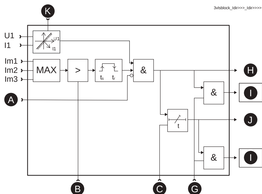
Figure 115 - Block diagram of directional phase overcurrent stage I\phi >>> and I\phi >>>>
