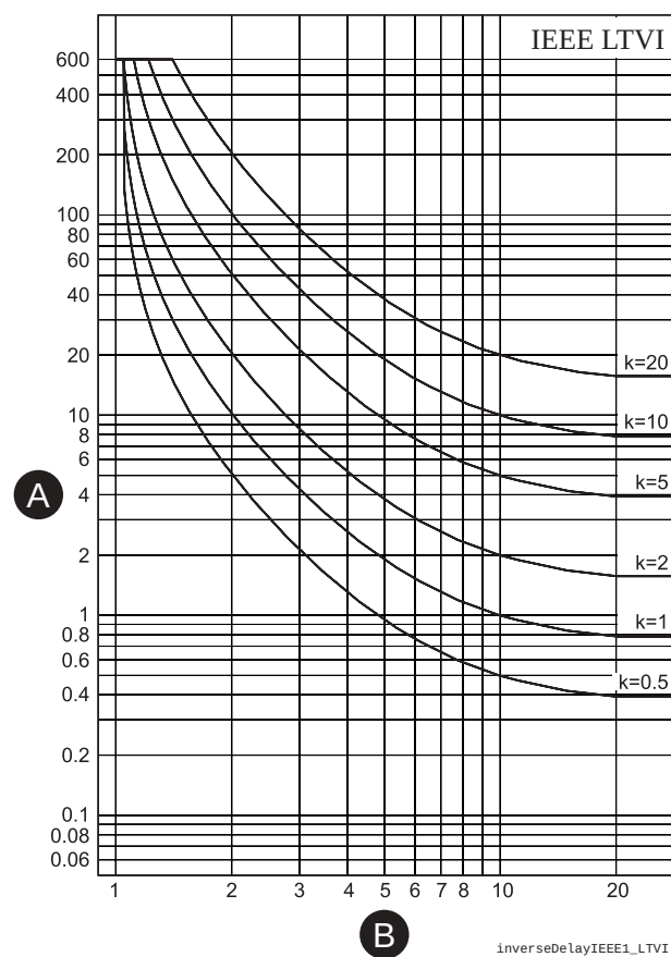
Figure 62 - ANSI/IEEE long time very inverse delay
