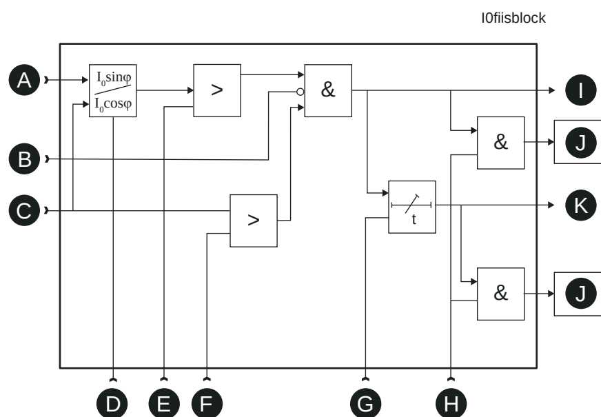
Figure 121 - Block diagram of the directional earth fault overcurrent stages I_{0\phi}> , I_{0\phi}>> , I_{0\phi}>>> , and I_{0\phi}>>>>
