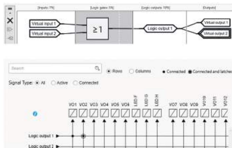
Figure 21 - Virtual inputs and outputs assigned to outputs of logical operators
