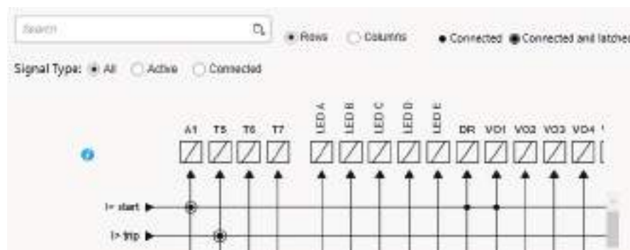
Figure 28 - Output matrix example view
