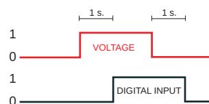
Figure 19 - Digital input's behavior when delay is set to 1 second
