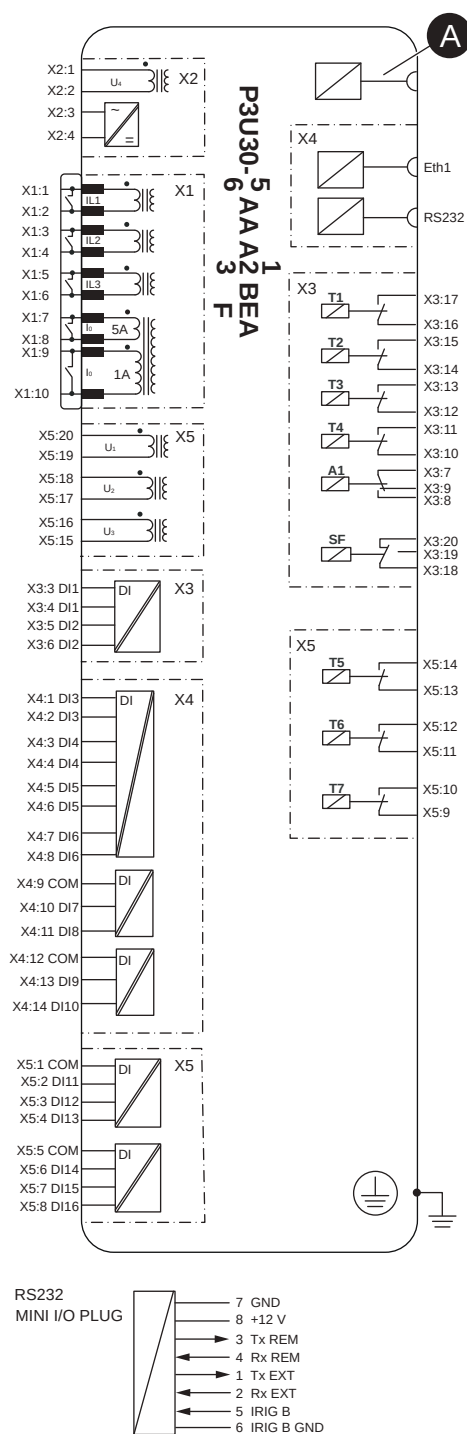
Figure 222 - P3U30 3AA A1 BEA block diagram
