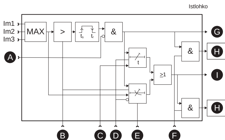
Figure 80 - Block diagram of motor start-up supervision I_{ST}
