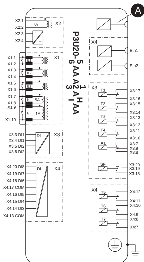
Figure 217 - P3U20 5AA A1AHAA block diagram
