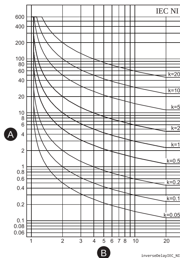
Figure 57 - IEC normal inverse delay
