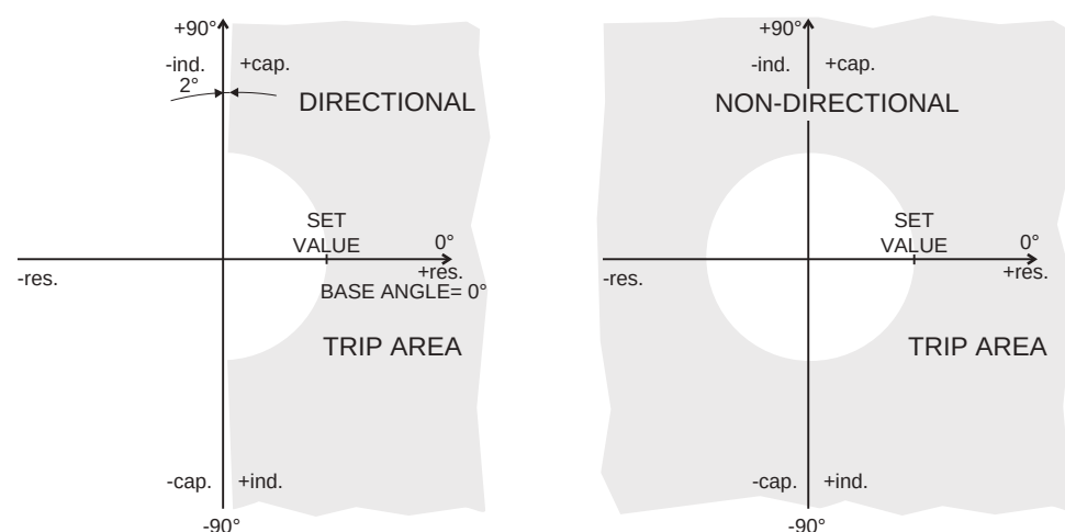
Figure 118 - Difference between directional and non-directional mode
