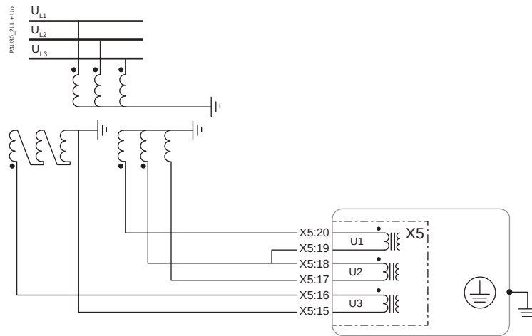
Figure 285 - 2LL+U 0
