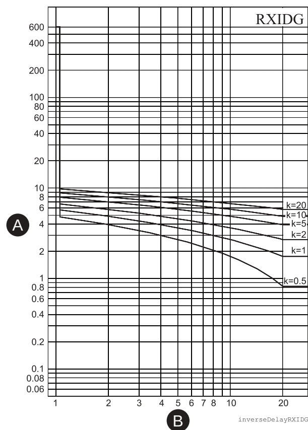
Figure 72 - RXIDG dependent delay
