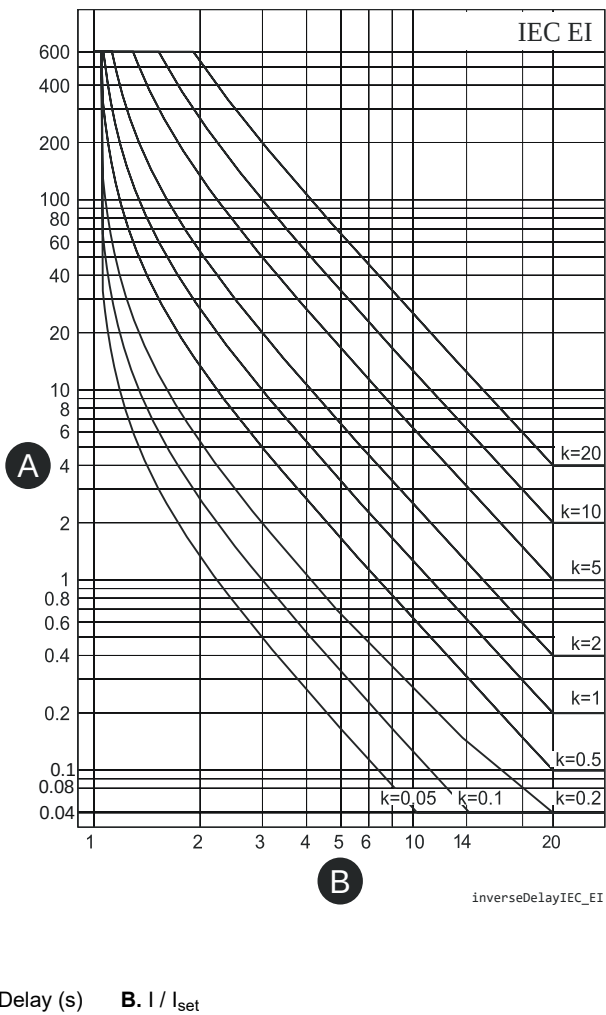
Figure 58 - IEC extremely inverse delay
