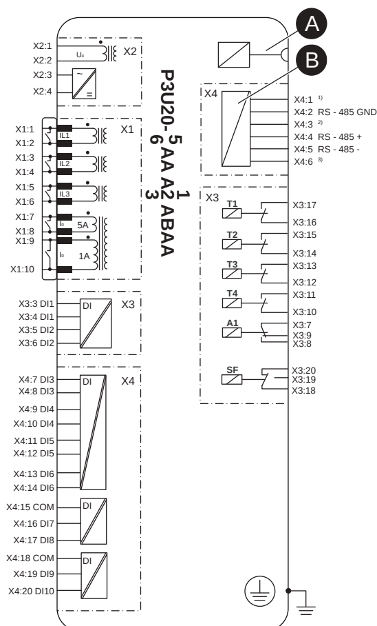
Figure 214 - P3U20 5AA A1ABAA block diagram
