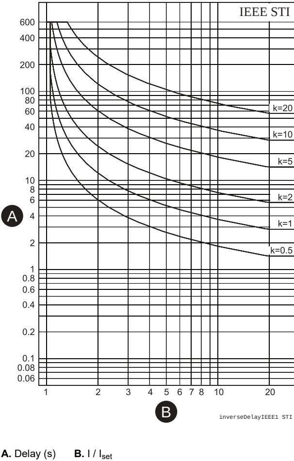
Figure 65 - ANSI/IEEE short time inverse delay
