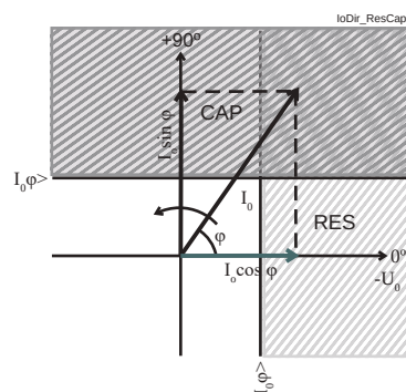
Figure 122 - Operation characteristics of the directional earth fault protection in Res and Cap mode
