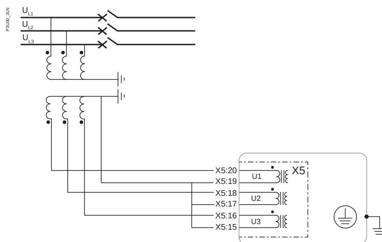
Figure 281 - 3LN
