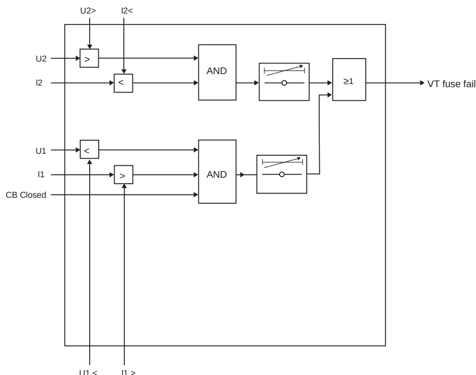
Figure 148 - Block diagram of 3-phase voltage transformer supervision
