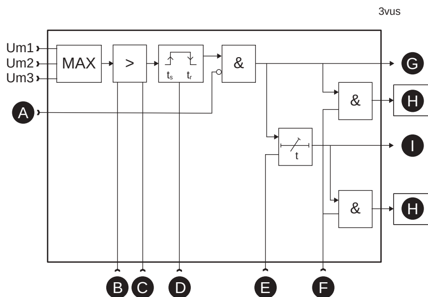
Figure 109 - Block diagram of the three-phase overvoltage stages U>, U>> and U>>>
