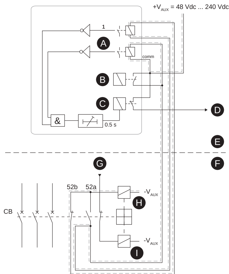
Figure 172 - Trip circuit supervision with two digital inputs and CB in open position
