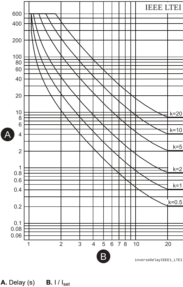
Figure 63 - ANSI/IEEE long time extremely inverse delay
