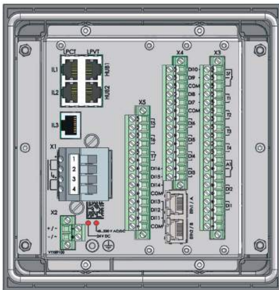
Figure 207 - P3U real panel – LPIT
