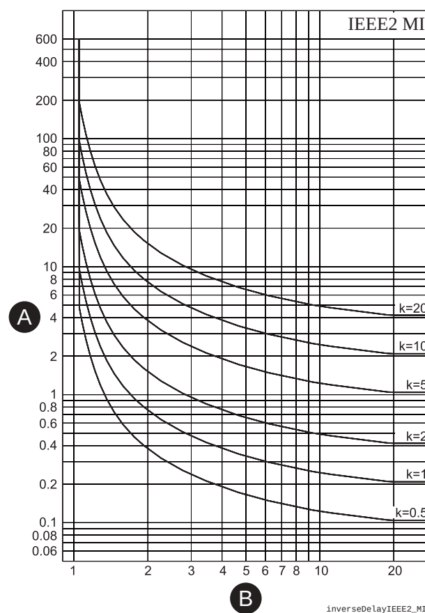
Figure 67 - IEEE2 moderately inverse delay
