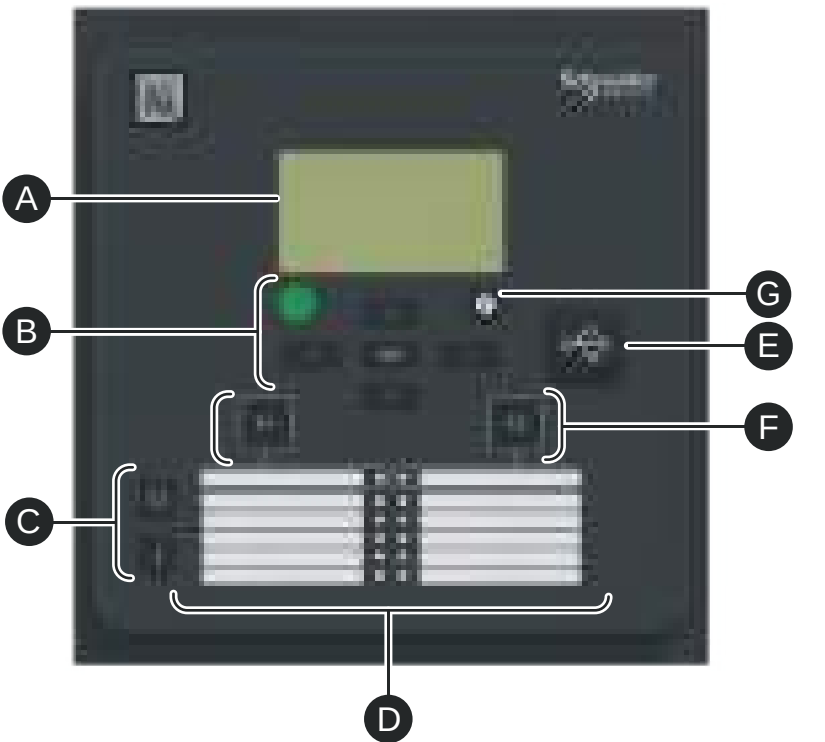
Figure 2 - PowerLogic P3U20 and P3U30 front panel
