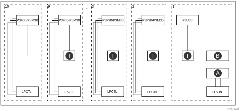
Figure 272 - LPVT sharing application without test sockets/plugs
