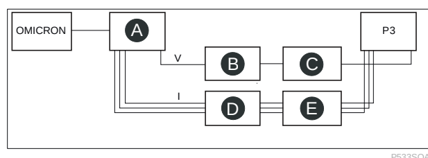
Figure 279 - LPCT/LPVT testing with test sockets/plugs
