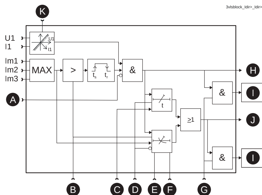
Figure 114 - Block diagram of directional phase overcurrent stage I\phi > and I\phi >>
