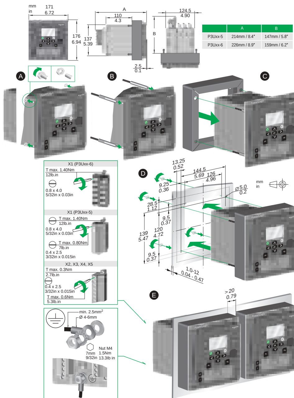
Figure 201 - Panel mounting with the raising frame REL52834
