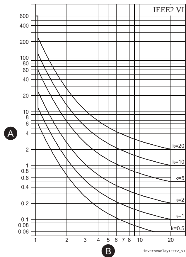
Figure 69 - IEEE2 very inverse delay
