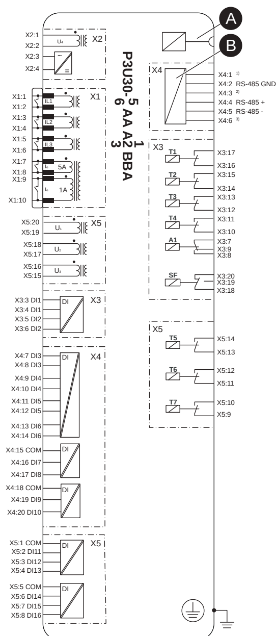
Figure 219 - P3U30 5AA A1BBA block diagram
