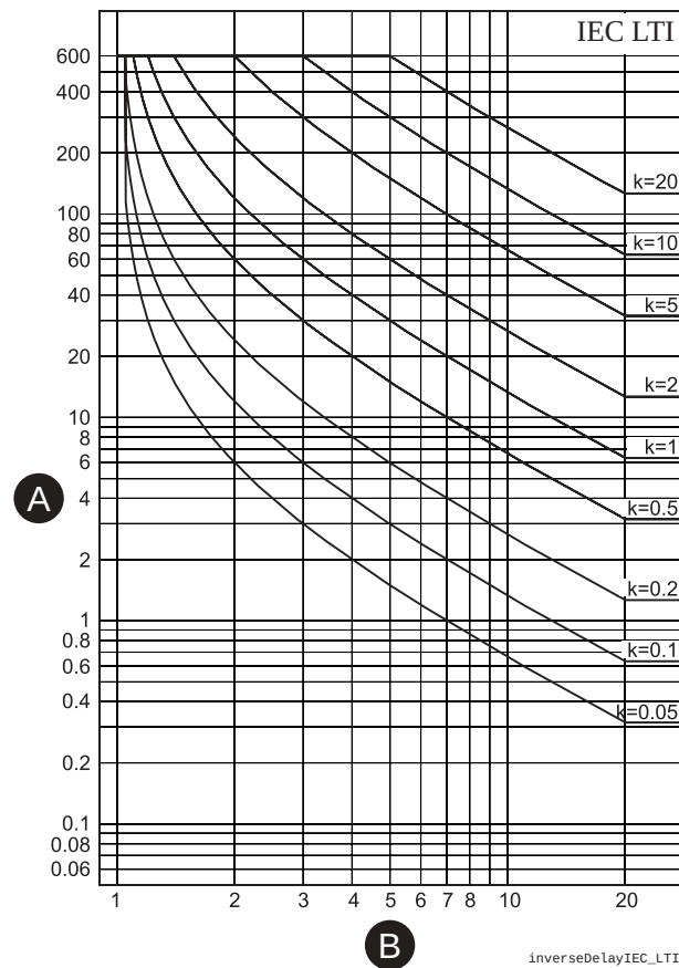
Figure 60 - IEC long time inverse delay
