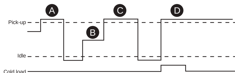
Figure 142 - Functionality of cold load / inrush current feature
