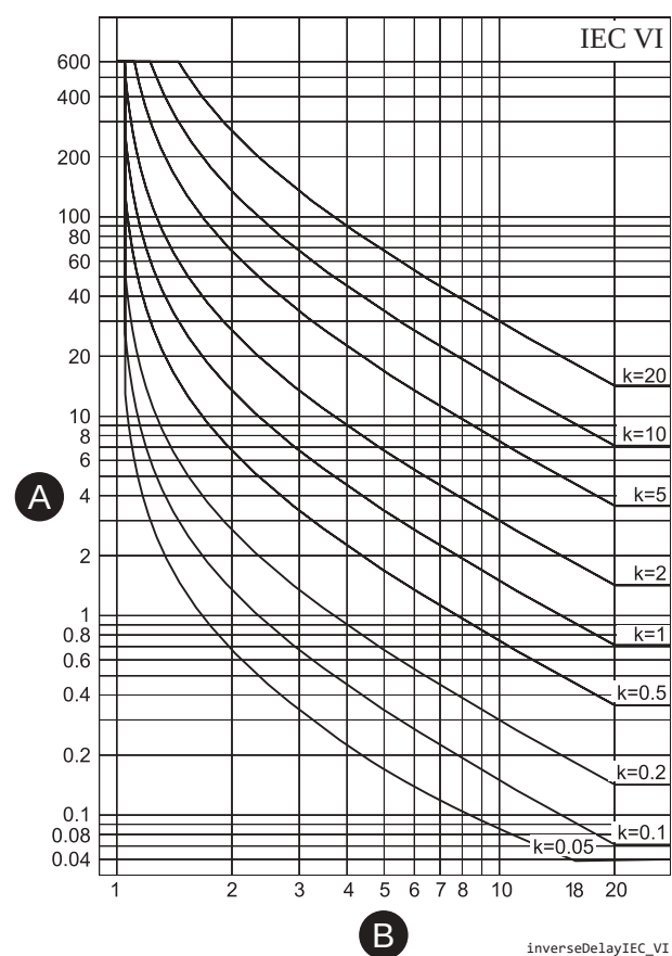
Figure 59 - IEC very inverse delay
