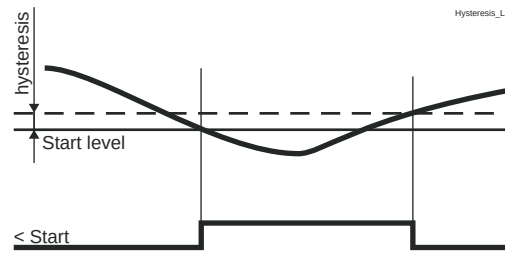
Figure 55 - Example behavior of an under-protection with hysteresis
