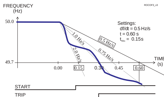
Figure 137 - An example of dependent df/dt operate time. The time to trip will be 0.3 s, although the setting is 0.6 s, because the average slope 1 Hz/s is steeper than the setting value 0.5 Hz/s.
