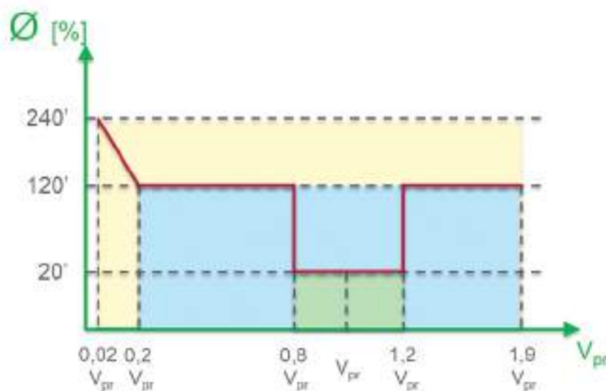
Figure 260 - Phase accuracy
