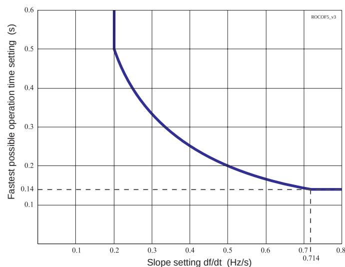
Figure 135 - At very sensitive slope settings the fastest possible operate time is limited.
