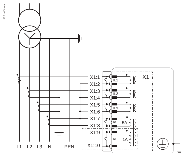
Figure 230 - Earth fault overcurrent measurement by sum of phase overcurrent and earth fault overcurrent
