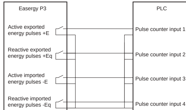
Figure 159 - Application example of wiring the energy pulse outputs to a PLC having common minus and an internal wetting voltage.
