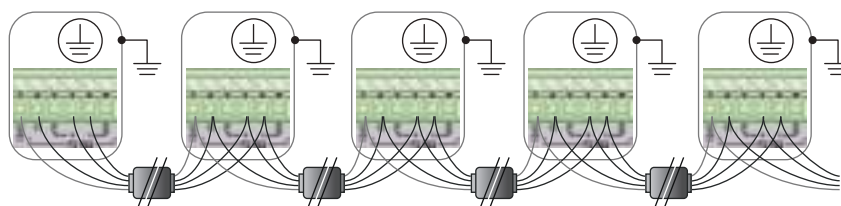
Figure 209 - RS-485 multidrop connections
