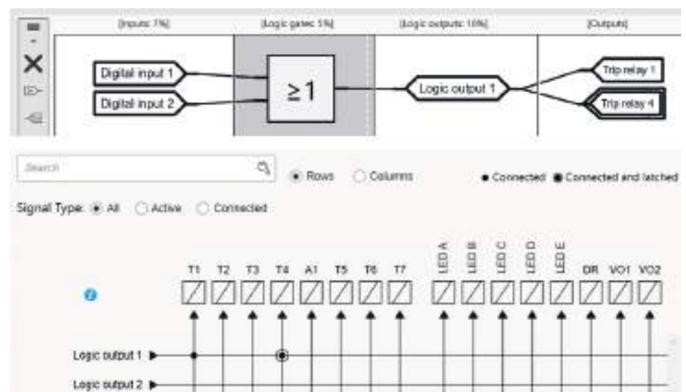
Figure 16 - Digital inputs assigned to outputs of logical operators
