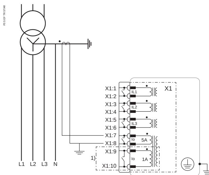
Figure 229 - Earth fault overcurrent measured from neutral earthing
