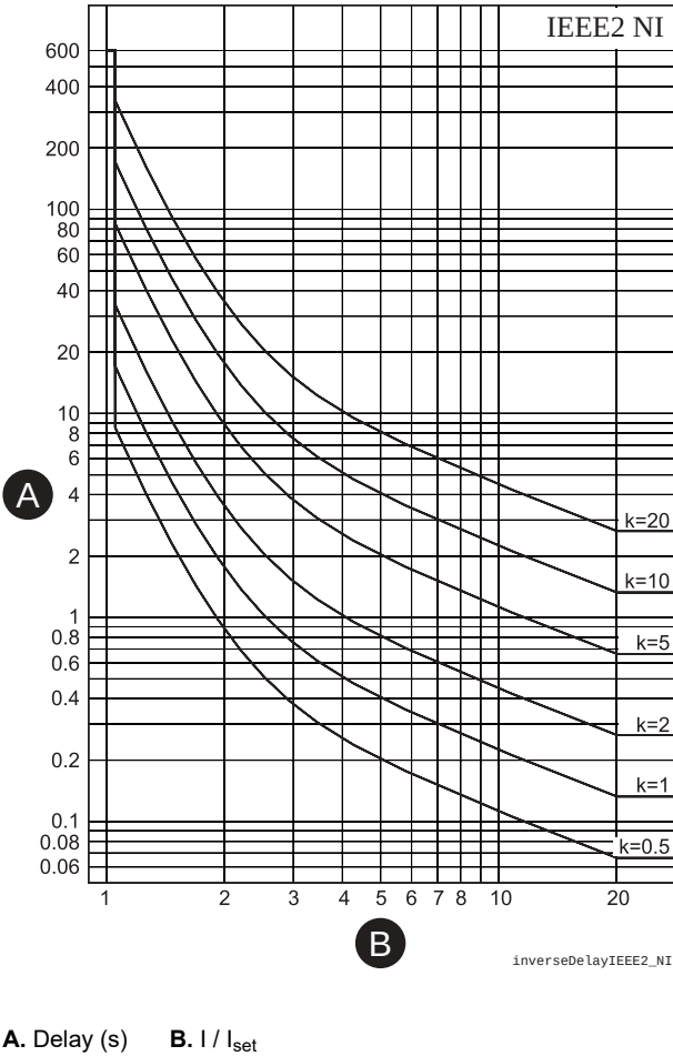
Figure 68 - IEEE2 normal inverse delay
