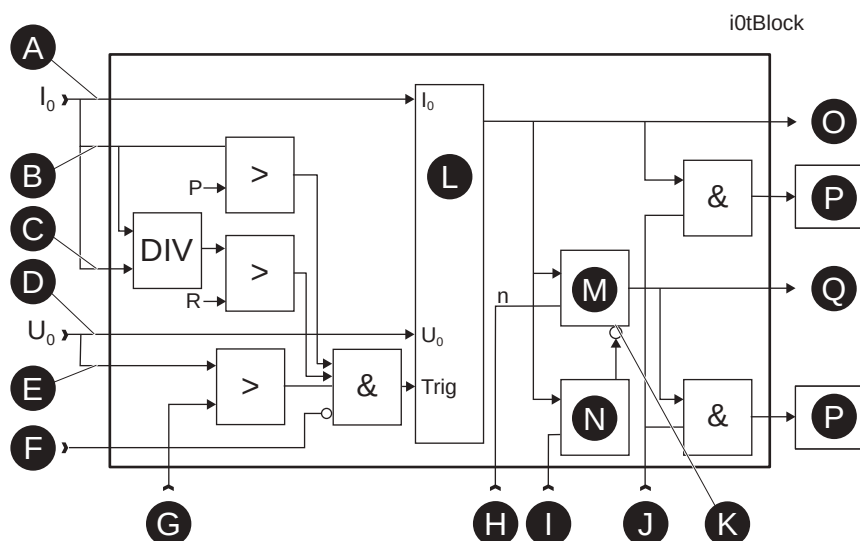
Figure 128 - Block diagram of the directional transient intermittent earth fault stage I_{0INT}>
