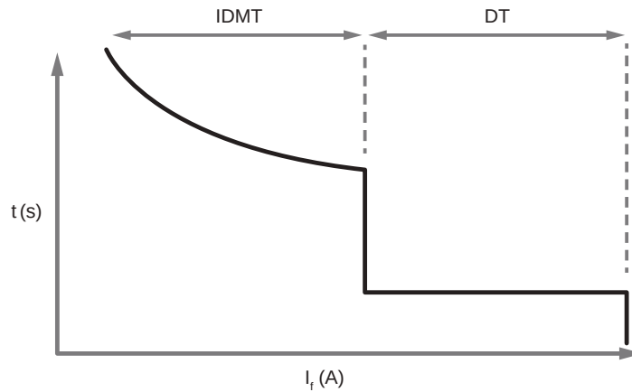
Figure 51 - Dependent time and definite time operation curves
