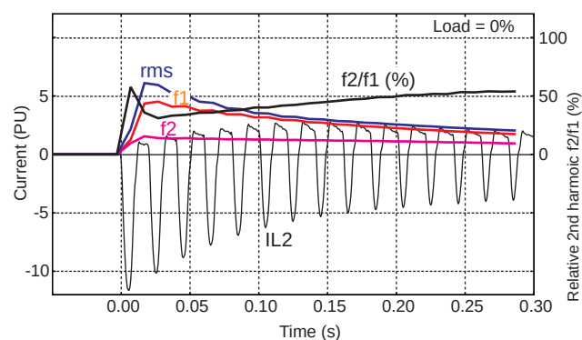
Figure 5 - Example of various current values of a transformer inrush current
