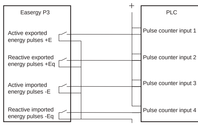
Figure 157 - Application example of wiring the energy pulse outputs to a PLC having common plus and using an external wetting voltage
