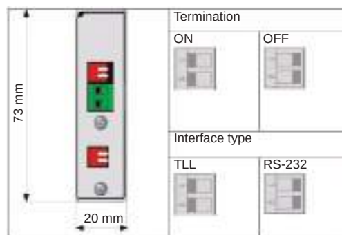
Figure 212 - RS-232 and TTL interface
