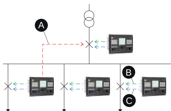
Figure 88 - CBFP implementation
