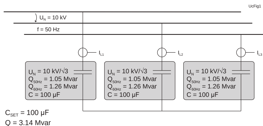
Figure 110 - Capacitor bank built of three single-phase units connected in wye (III Y). Each capacitor is 100 \mu F and this value is also used as the setting value.
