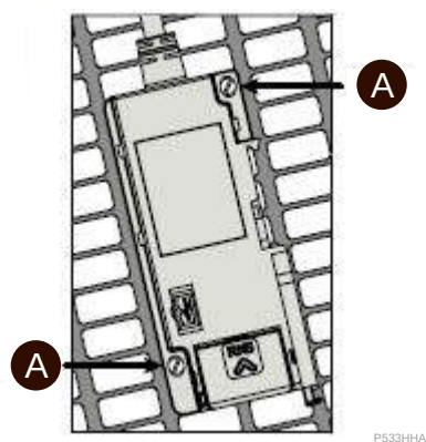
Figure 246 - Mounting on Telequick grid
