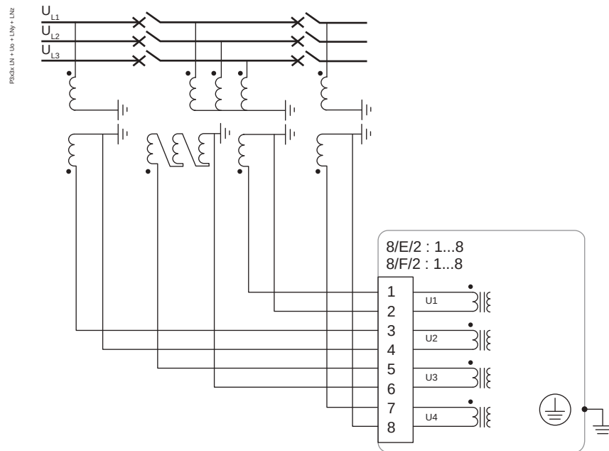
Figure 291 - LN+U 0 +LNy+LNz
