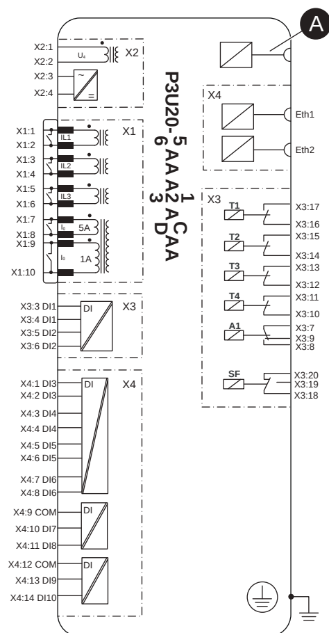
Figure 215 - P3U20 5AA A1ACAA block diagram
