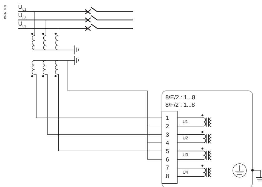
Figure 290 - 3LN
