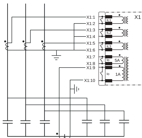
Figure 98 - Typical capacitor bank protection application with PowerLogic P3 relays
