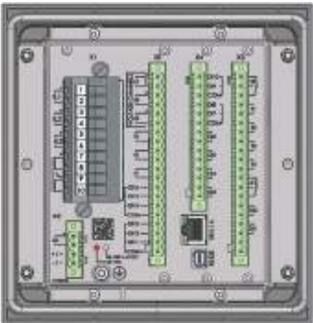
Figure 204 - Pluggable Clamp RJ45 ETH_RS232 without X2-X5 connectors P3Uxx-5ABA1BEA
