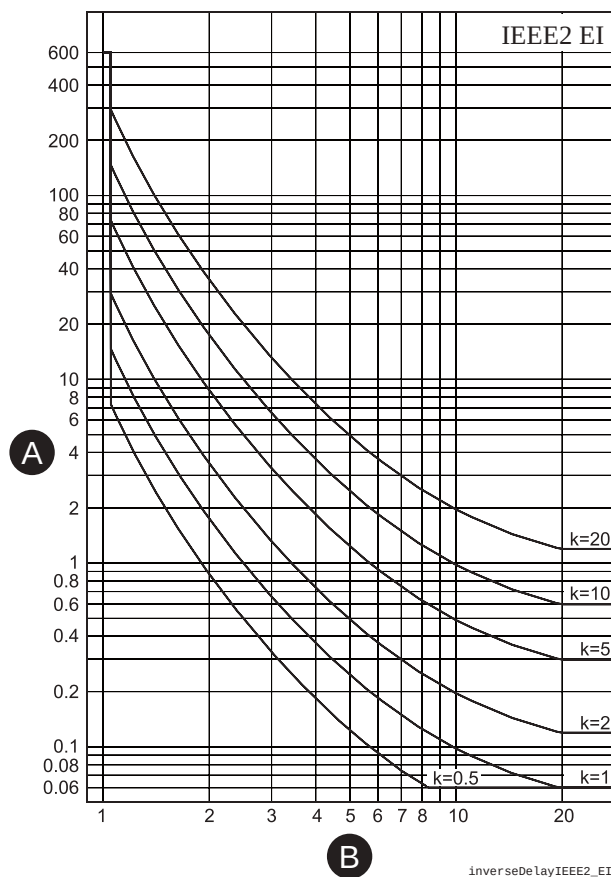
Figure 70 - IEEE2 extremely inverse delay
