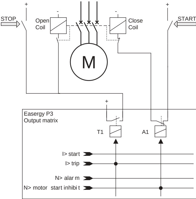
Figure 113 - Application for preventing too frequent starting using the N> stage
