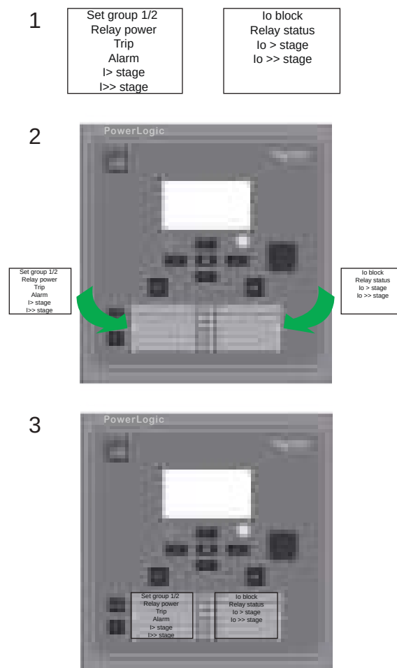
Figure 202 - Example of the P3U alarm facial label insertion
