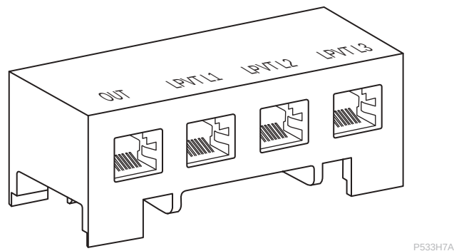
Figure 238 - LPVT hub connector
