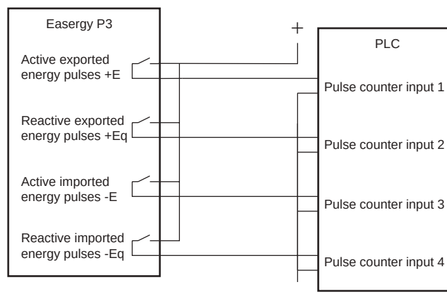
Figure 158 - Application example of wiring the energy pulse outputs to a PLC having common minus and using an external wetting voltage
