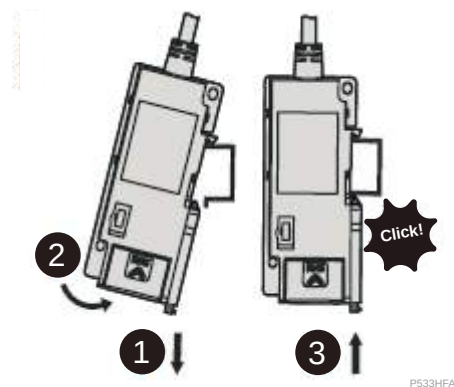
Figure 244 - Mounting on DIN rail
