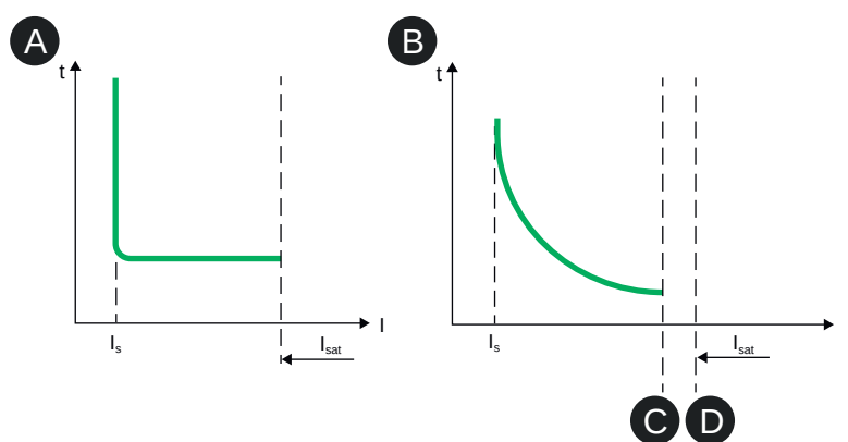
Figure 45 - Overcurrent characteristics
