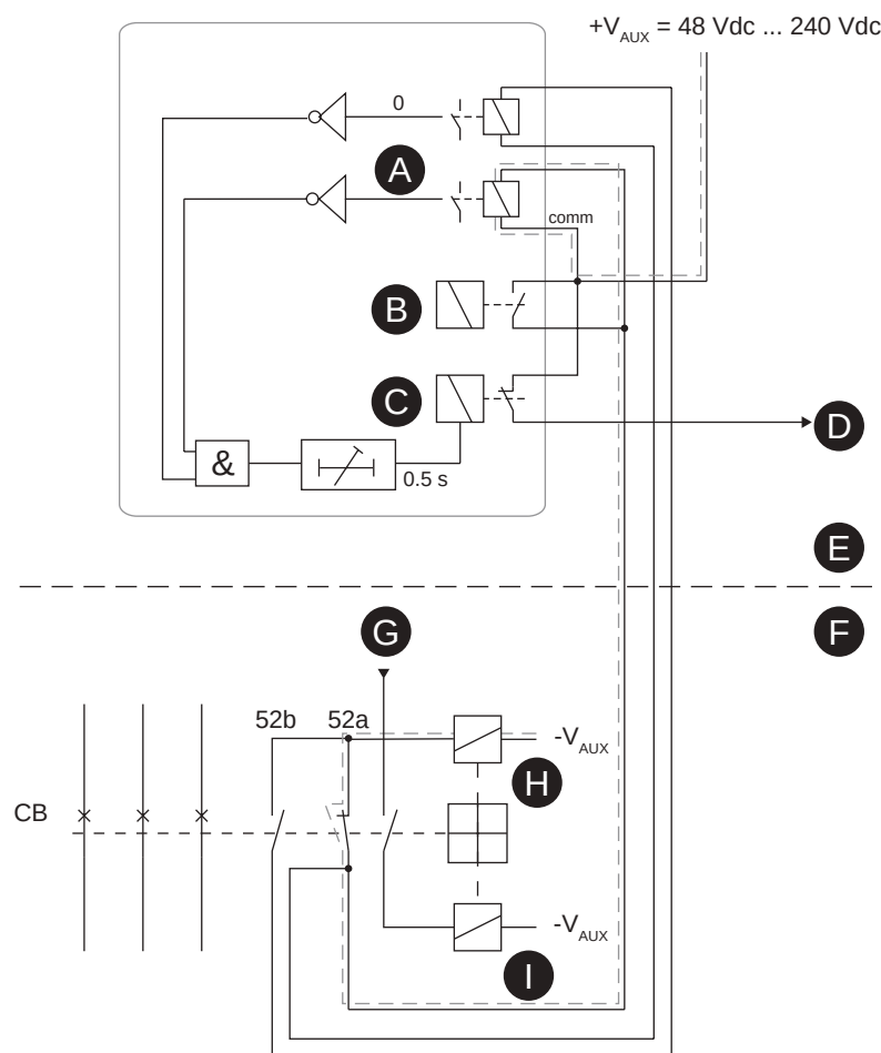
Figure 171 - Trip circuit supervision with two digital inputs and closed CB
