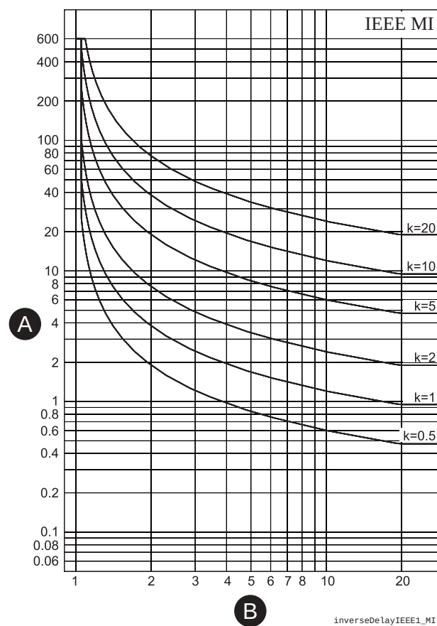
Figure 64 - ANSI/IEEE moderately inverse delay
