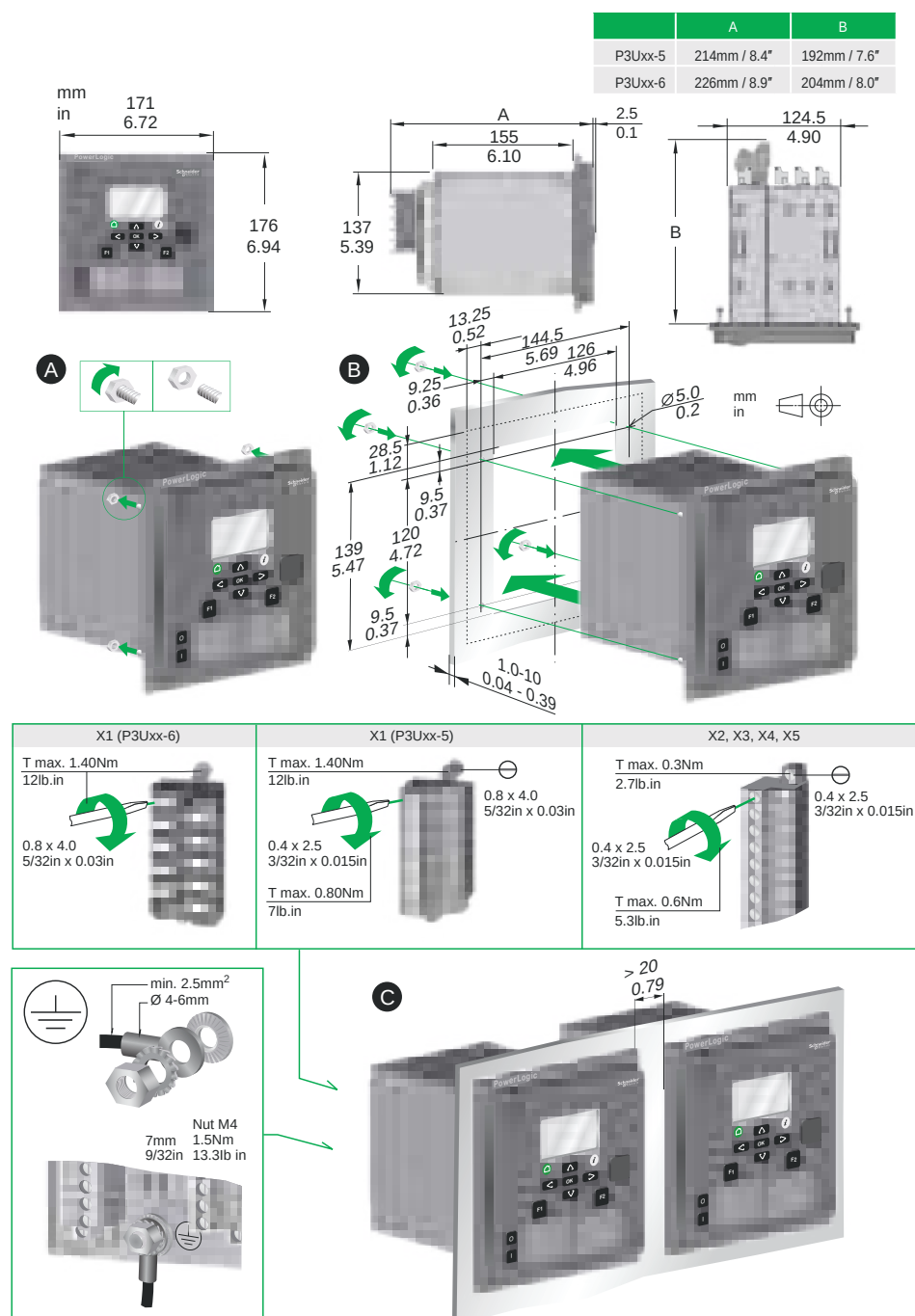
Figure 200 - Panel mounting
