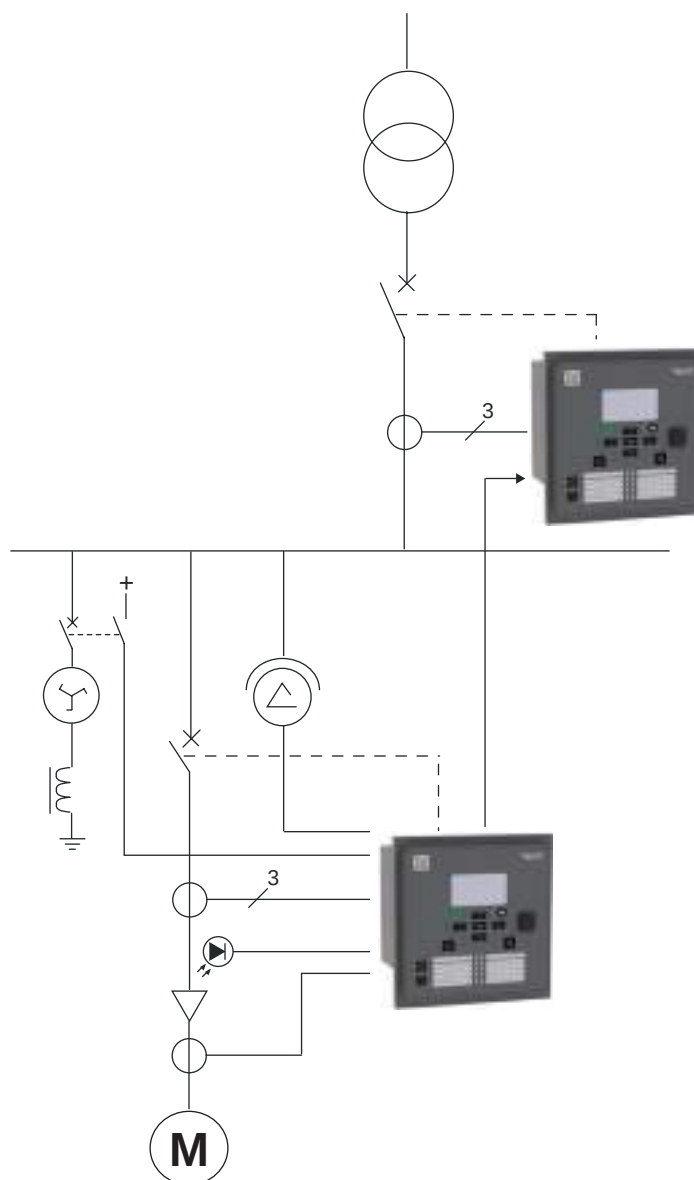
Figure 192 - PowerLogic P3U20 and P3U30 used in cable protection of an industry plant network.
