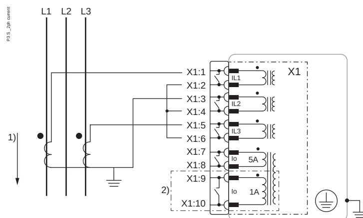
Figure 224 - Two-phase current measurement
